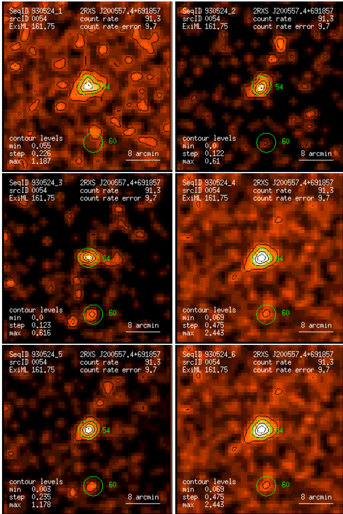
Figure 54: RASS 930524: detection 0054: band rate images, Gaussian filter: (1) PSPC channels 11 – 41, (2) 52 – 90, (3) 91 – 201, (4) 11 – 235, (5) 52 – 201, (6) 11 – 201. Broad band rates in counts/ks. Band rate contour levels in counts/ks/arcmin 2 .
