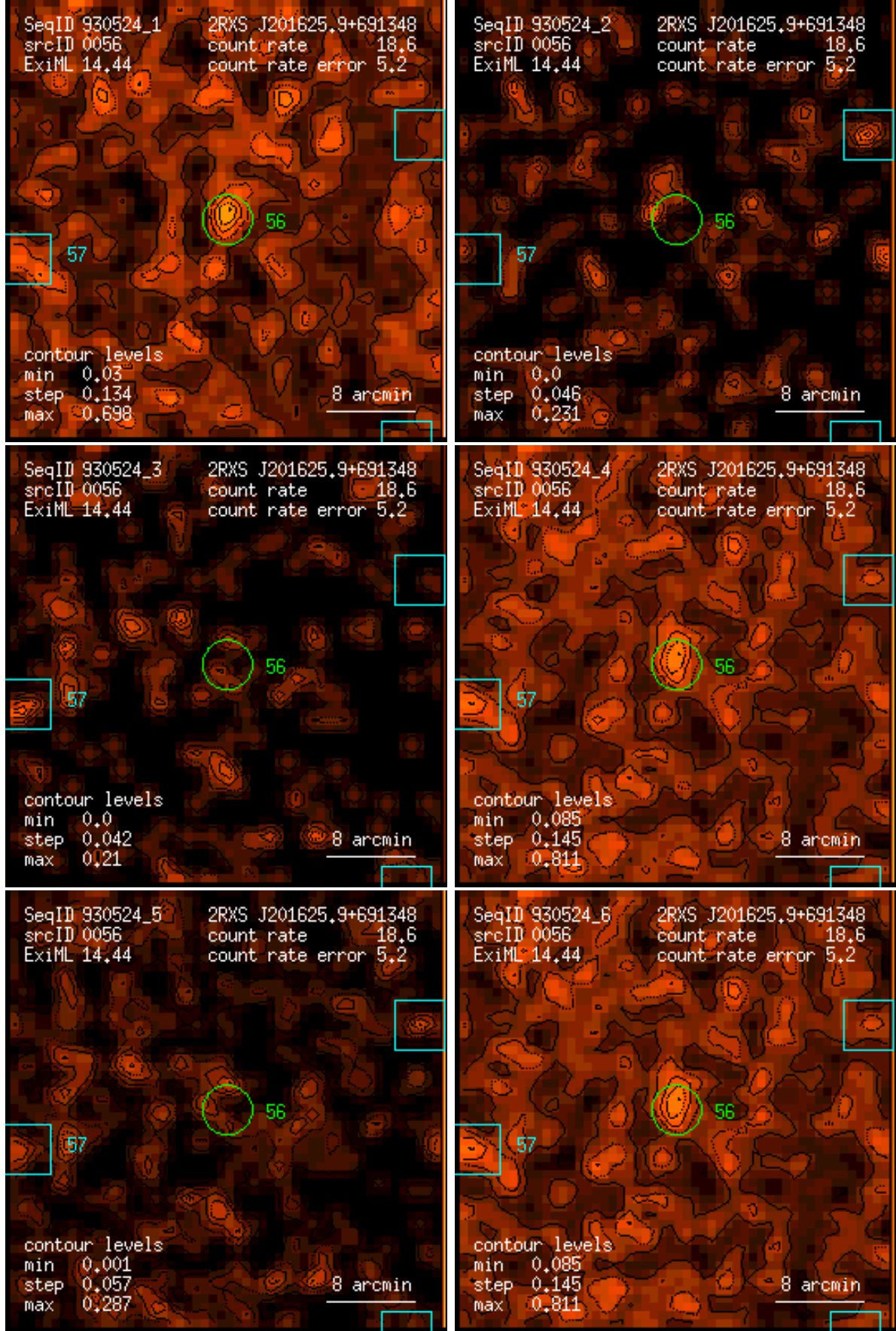
Figure 56: RASS 930524: detection 0056: band rate images, Gaussian filter: (1) PSPC channels 11 – 41, (2) 52 – 90, (3) 91 – 201, (4) 11 – 235, (5) 52 – 201, (6) 11 – 201. Broad band rates in counts/ks. Band rate contour levels in counts/ks/arcmin 2 .
