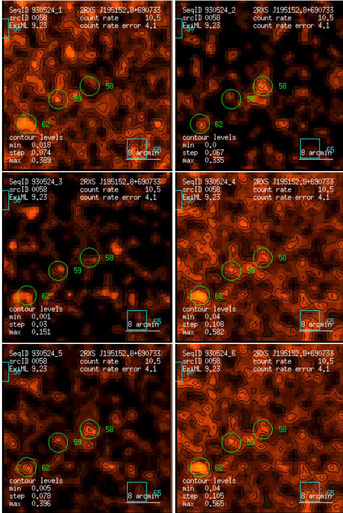
Figure 58: RASS 930524: detection 0058: band rate images, Gaussian filter: (1) PSPC channels 11 – 41, (2) 52 – 90, (3) 91 – 201, (4) 11 – 235, (5) 52 – 201, (6) 11 – 201. Broad band rates in counts/ks. Band rate contour levels in counts/ks/arcmin 2 .
