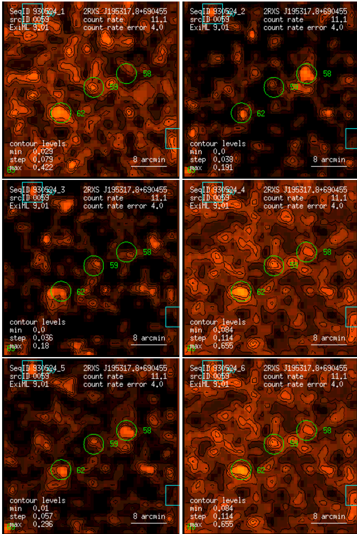
Figure 59: RASS 930524: detection 0059: band rate images, Gaussian filter: (1) PSPC channels 11 – 41, (2) 52 – 90, (3) 91 – 201, (4) 11 – 235, (5) 52 – 201, (6) 11 – 201. Broad band rates in counts/ks. Band rate contour levels in counts/ks/arcmin 2 .
