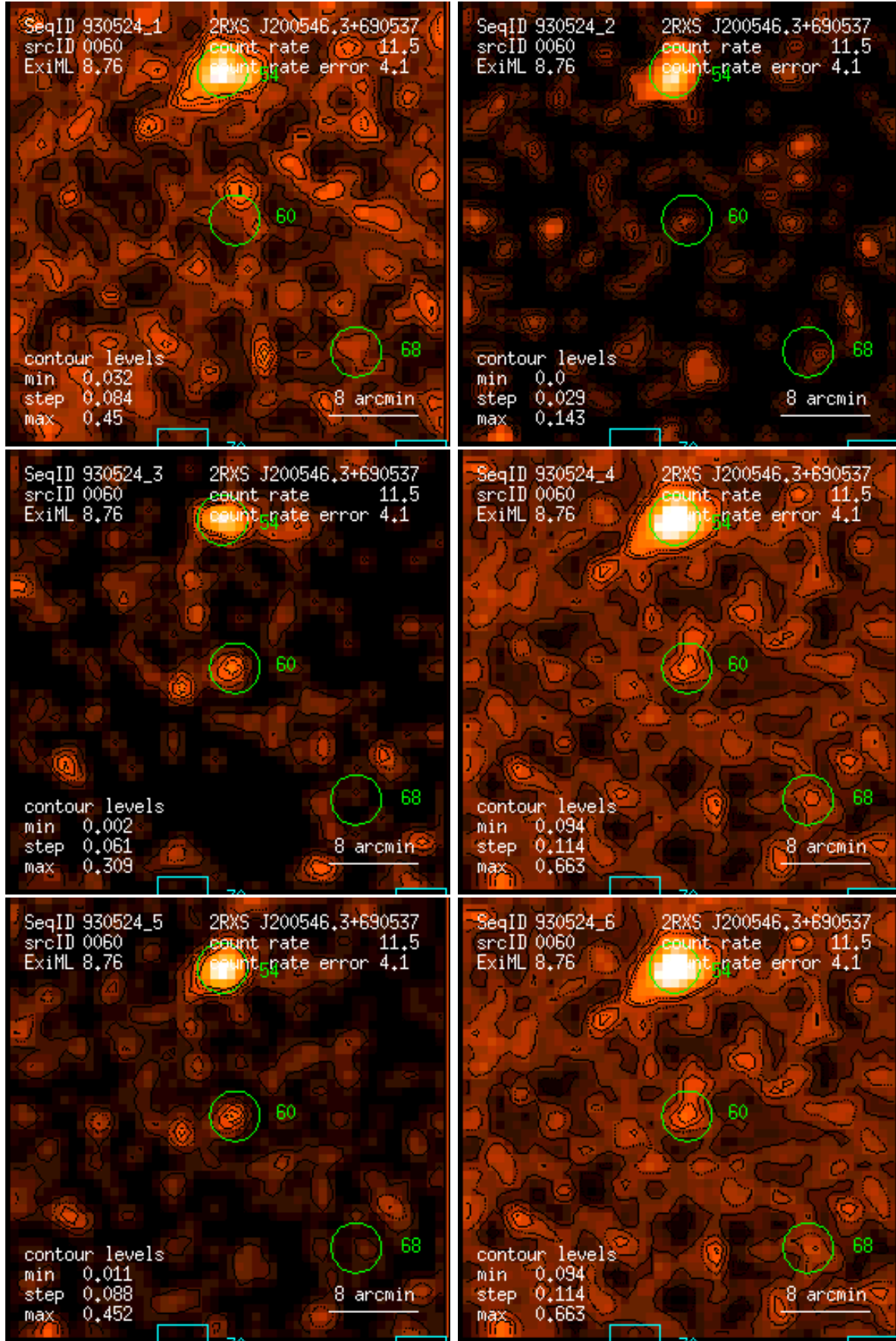
Figure 60: RASS 930524: detection 0060: band rate images, Gaussian filter: (1) PSPC channels 11 – 41, (2) 52 – 90, (3) 91 – 201, (4) 11 – 235, (5) 52 – 201, (6) 11 – 201. Broad band rates in counts/ks. Band rate contour levels in counts/ks/arcmin 2 .
