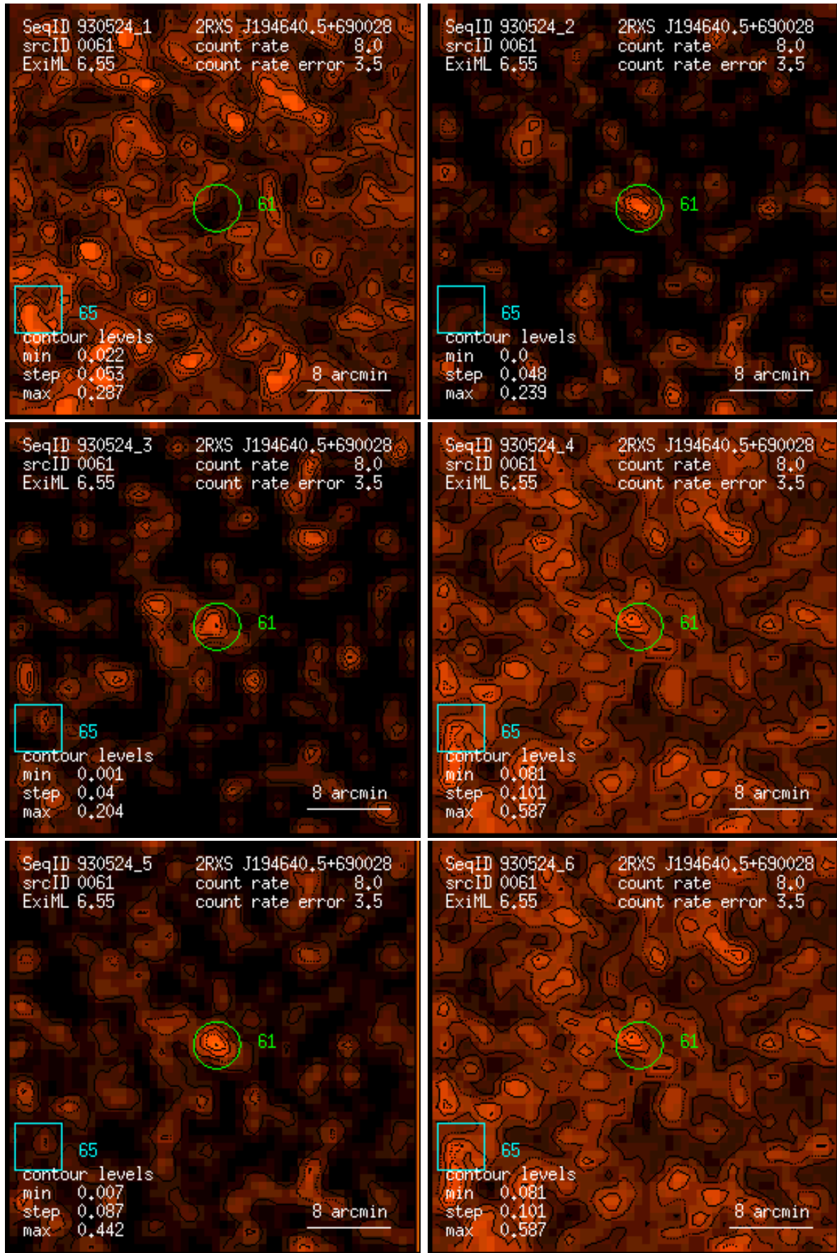
Figure 61: RASS 930524: detection 0061: band rate images, Gaussian filter: (1) PSPC channels 11 – 41, (2) 52 – 90, (3) 91 – 201, (4) 11 – 235, (5) 52 – 201, (6) 11 – 201. Broad band rates in counts/ks. Band rate contour levels in counts/ks/arcmin 2 .
