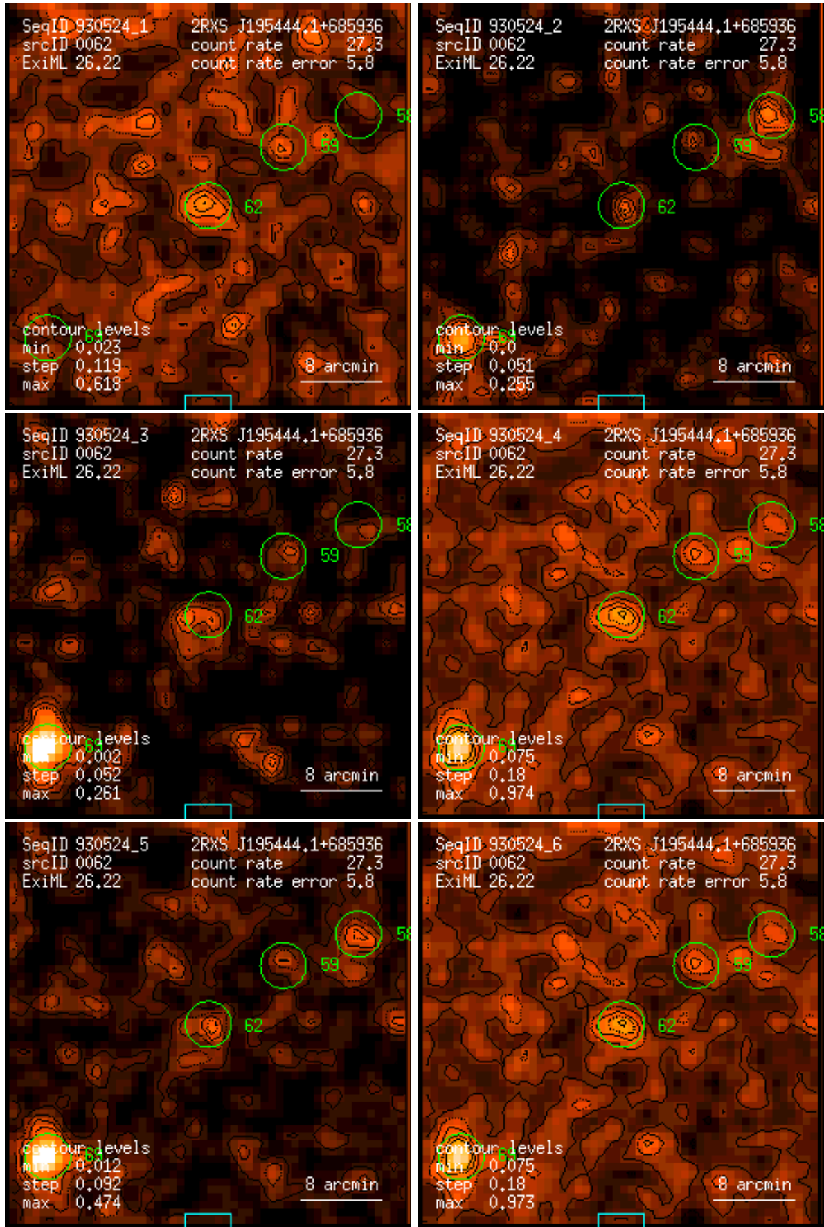
Figure 62: RASS 930524: detection 0062: band rate images, Gaussian filter: (1) PSPC channels 11 – 41, (2) 52 – 90, (3) 91 – 201, (4) 11 – 235, (5) 52 – 201, (6) 11 – 201. Broad band rates in counts/ks. Band rate contour levels in counts/ks/arcmin 2 .
