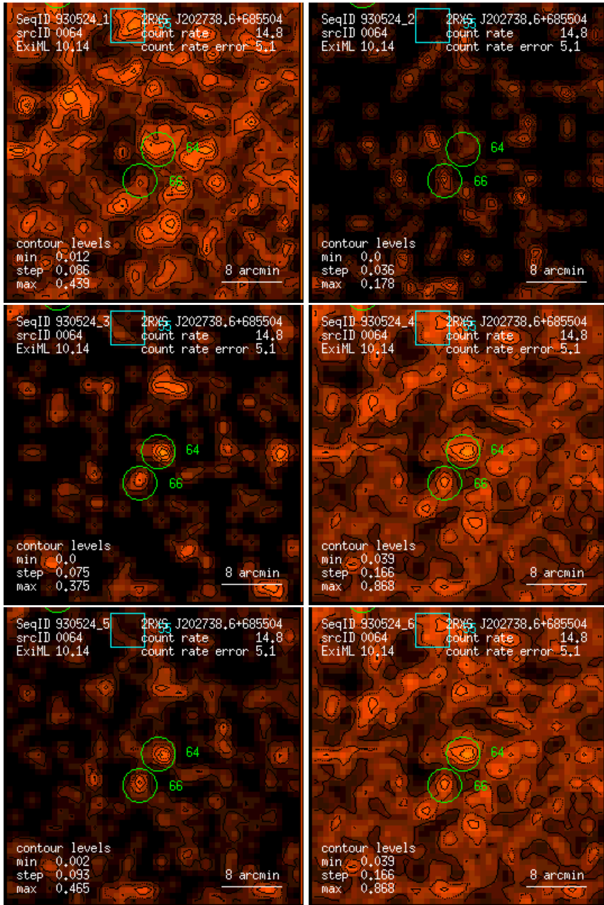
Figure 64: RASS 930524: detection 0064: band rate images, Gaussian filter: (1) PSPC channels 11 – 41, (2) 52 – 90, (3) 91 – 201, (4) 11 – 235, (5) 52 – 201, (6) 11 – 201. Broad band rates in counts/ks. Band rate contour levels in counts/ks/arcmin 2 .
