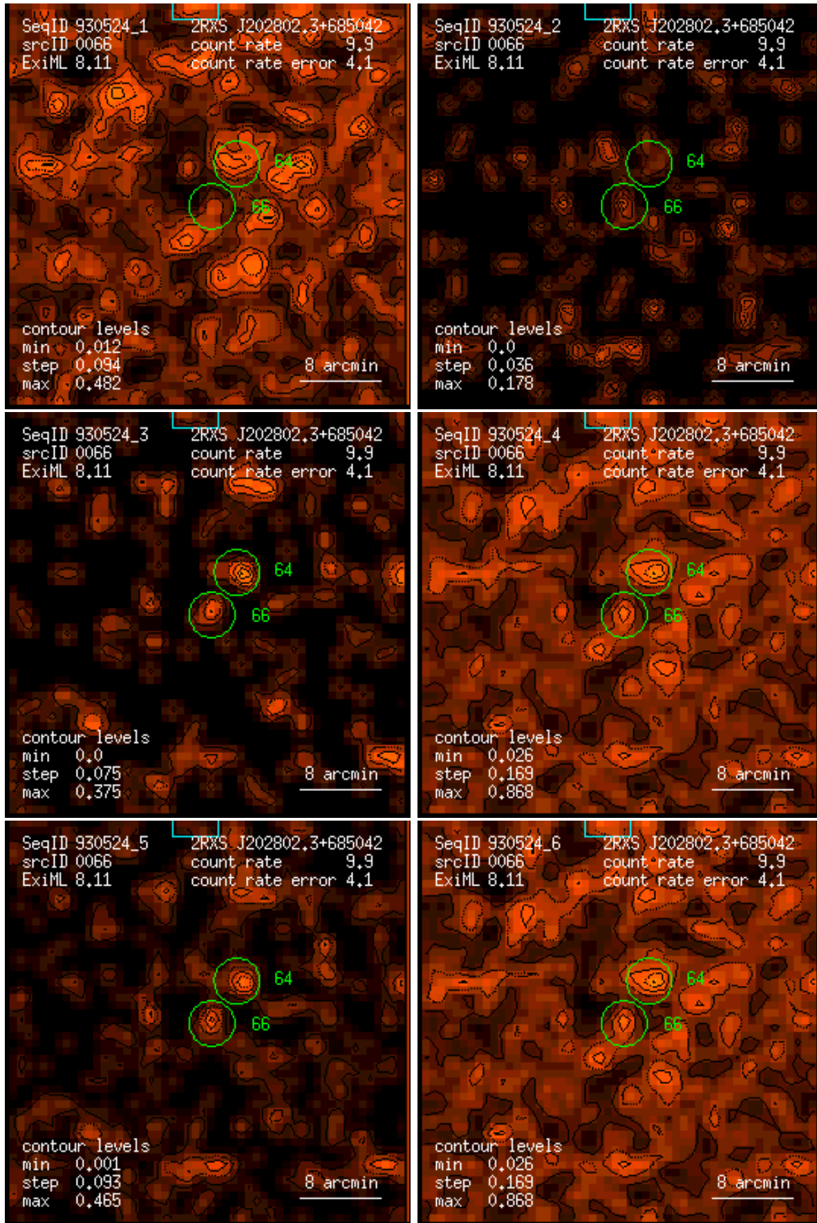
Figure 66: RASS 930524: detection 0066: band rate images, Gaussian filter: (1) PSPC channels 11 – 41, (2) 52 – 90, (3) 91 – 201, (4) 11 – 235, (5) 52 – 201, (6) 11 – 201. Broad band rates in counts/ks. Band rate contour levels in counts/ks/arcmin 2 .
