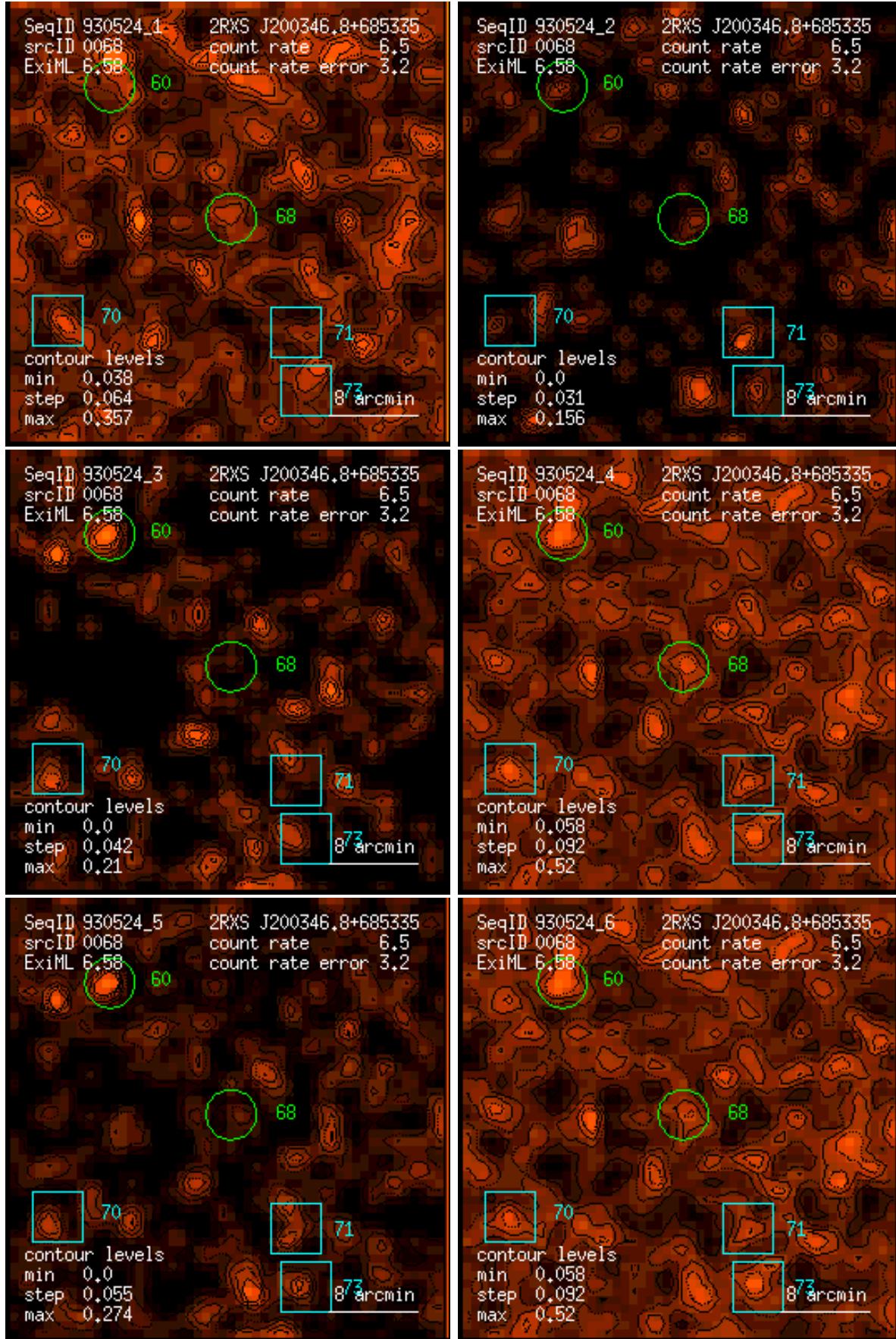
Figure 68: RASS 930524: detection 0068: band rate images, Gaussian filter: (1) PSPC channels 11 – 41, (2) 52 – 90, (3) 91 – 201, (4) 11 – 235, (5) 52 – 201, (6) 11 – 201. Broad band rates in counts/ks. Band rate contour levels in counts/ks/arcmin 2 .
