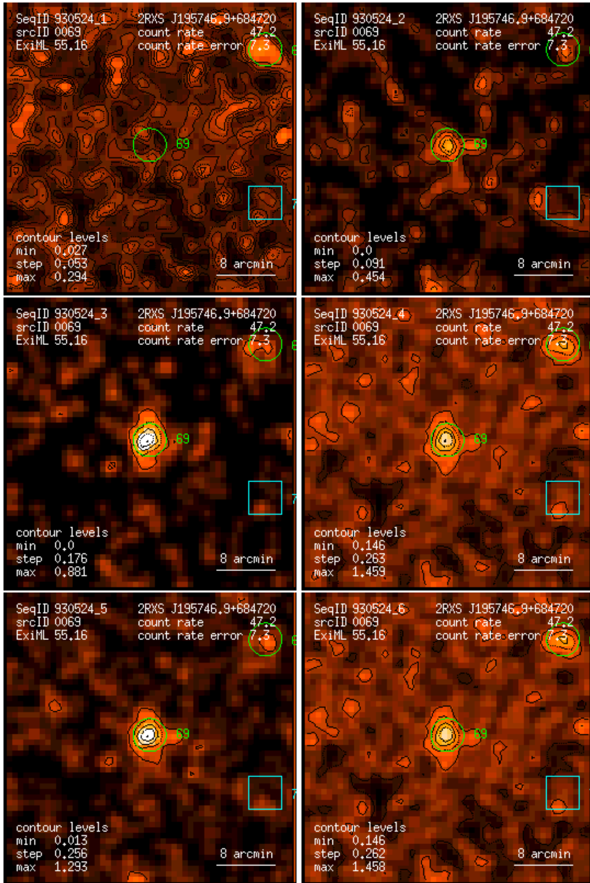
Figure 69: RASS 930524: detection 0069: band rate images, Gaussian filter: (1) PSPC channels 11 – 41, (2) 52 – 90, (3) 91 – 201, (4) 11 – 235, (5) 52 – 201, (6) 11 – 201. Broad band rates in counts/ks. Band rate contour levels in counts/ks/arcmin 2 .
