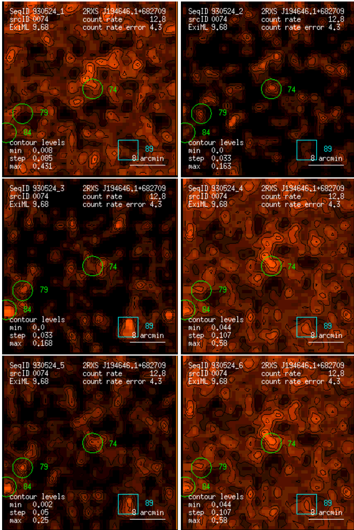
Figure 74: RASS 930524: detection 0074: band rate images, Gaussian filter: (1) PSPC channels 11 – 41, (2) 52 – 90, (3) 91 – 201, (4) 11 – 235, (5) 52 – 201, (6) 11 – 201. Broad band rates in counts/ks. Band rate contour levels in counts/ks/arcmin 2 .
