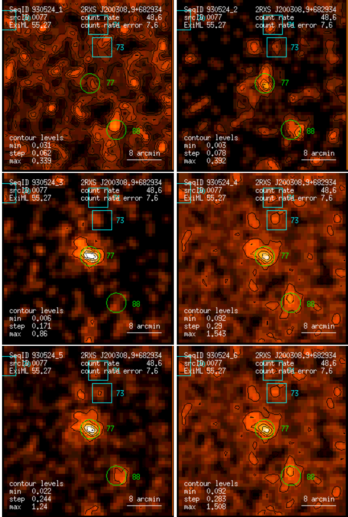
Figure 77: RASS 930524: detection 0077: band rate images, Gaussian filter: (1) PSPC channels 11 – 41, (2) 52 – 90, (3) 91 – 201, (4) 11 – 235, (5) 52 – 201, (6) 11 – 201. Broad band rates in counts/ks. Band rate contour levels in counts/ks/arcmin 2 .
