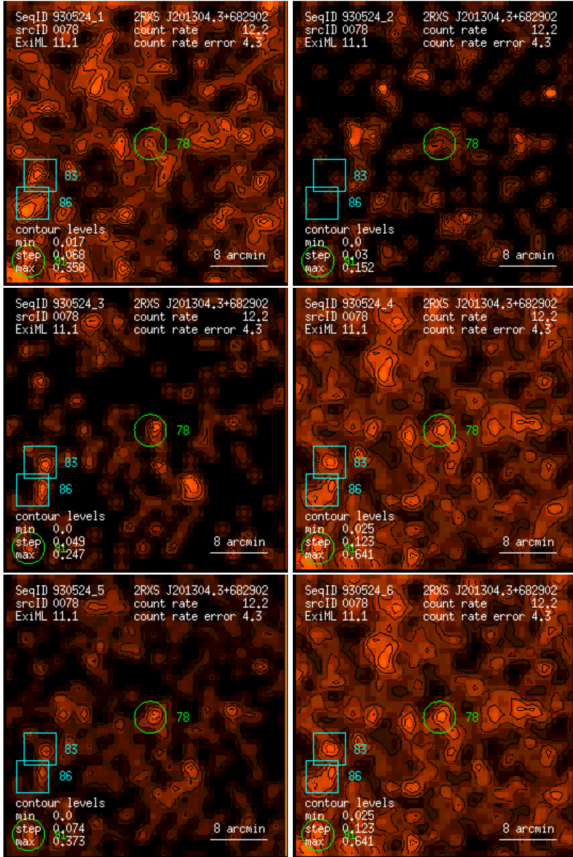
Figure 78: RASS 930524: detection 0078: band rate images, Gaussian filter: (1) PSPC channels 11 – 41, (2) 52 – 90, (3) 91 – 201, (4) 11 – 235, (5) 52 – 201, (6) 11 – 201. Broad band rates in counts/ks. Band rate contour levels in counts/ks/arcmin 2 .
