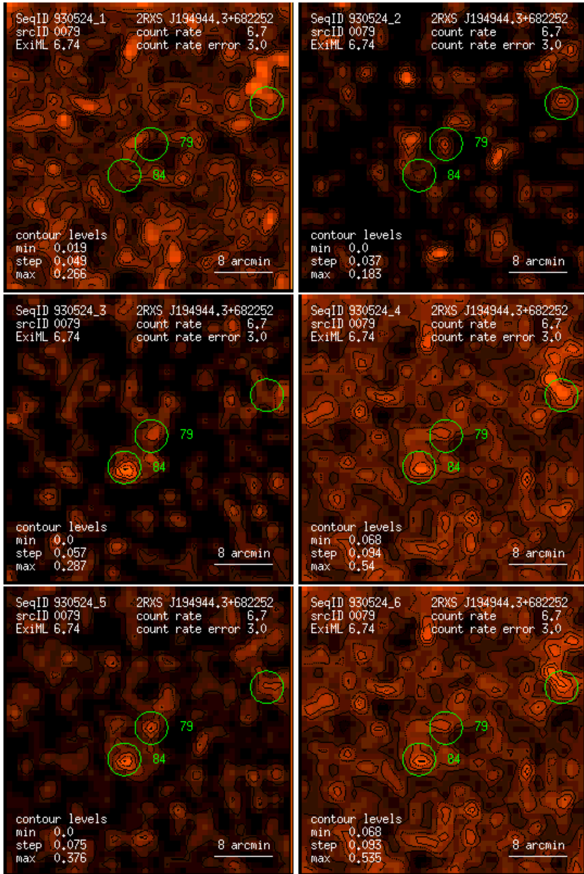
Figure 79: RASS 930524: detection 0079: band rate images, Gaussian filter: (1) PSPC channels 11 – 41, (2) 52 – 90, (3) 91 – 201, (4) 11 – 235, (5) 52 – 201, (6) 11 – 201. Broad band rates in counts/ks. Band rate contour levels in counts/ks/arcmin 2 .
