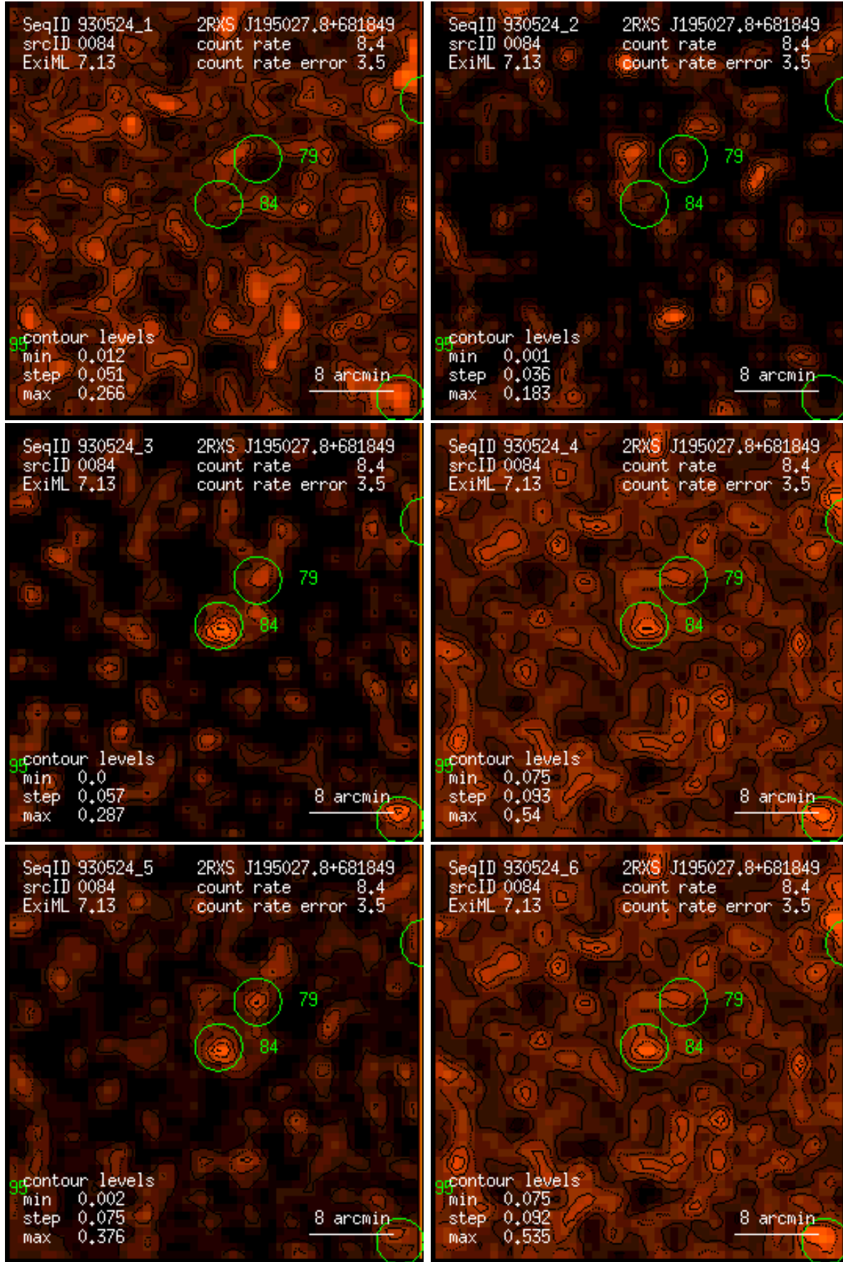
Figure 84: RASS 930524: detection 0084: band rate images, Gaussian filter: (1) PSPC channels 11 – 41, (2) 52 – 90, (3) 91 – 201, (4) 11 – 235, (5) 52 – 201, (6) 11 – 201. Broad band rates in counts/ks. Band rate contour levels in counts/ks/arcmin 2 .
