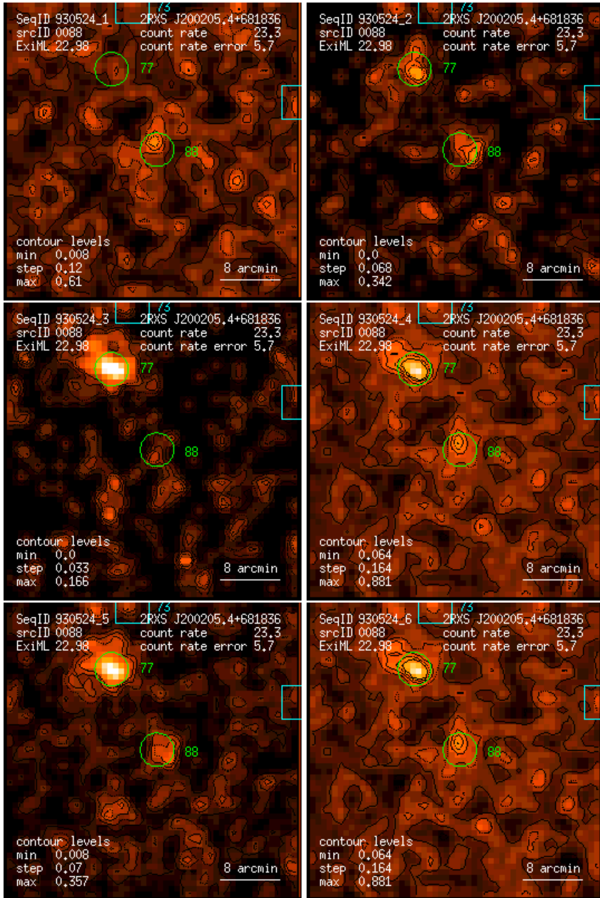
Figure 88: RASS 930524: detection 0088: band rate images, Gaussian filter: (1) PSPC channels 11 – 41, (2) 52 – 90, (3) 91 – 201, (4) 11 – 235, (5) 52 – 201, (6) 11 – 201. Broad band rates in counts/ks. Band rate contour levels in counts/ks/arcmin 2 .
