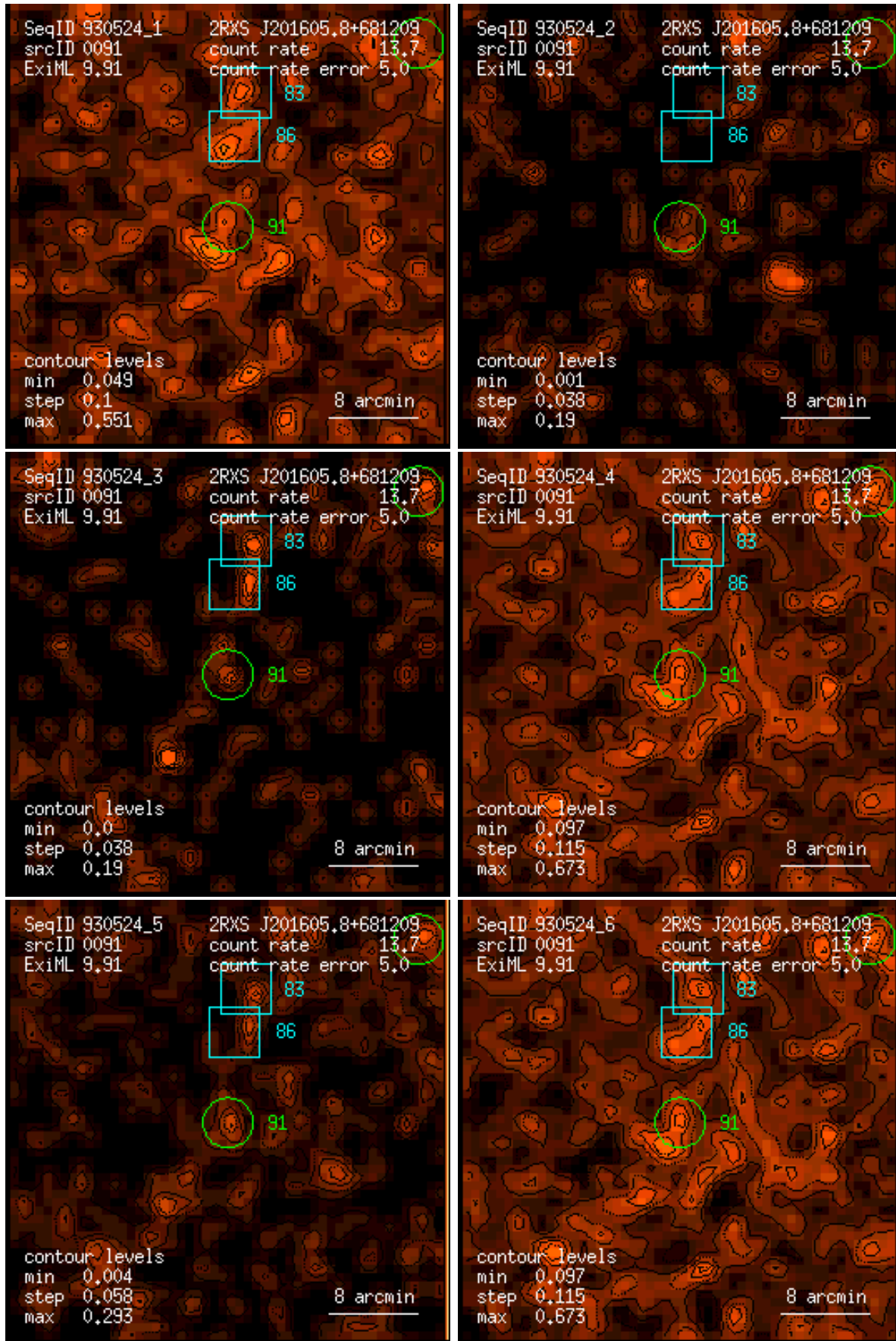
Figure 91: RASS 930524: detection 0091: band rate images, Gaussian filter: (1) PSPC channels 11 – 41, (2) 52 – 90, (3) 91 – 201, (4) 11 – 235, (5) 52 – 201, (6) 11 – 201. Broad band rates in counts/ks. Band rate contour levels in counts/ks/arcmin 2 .
