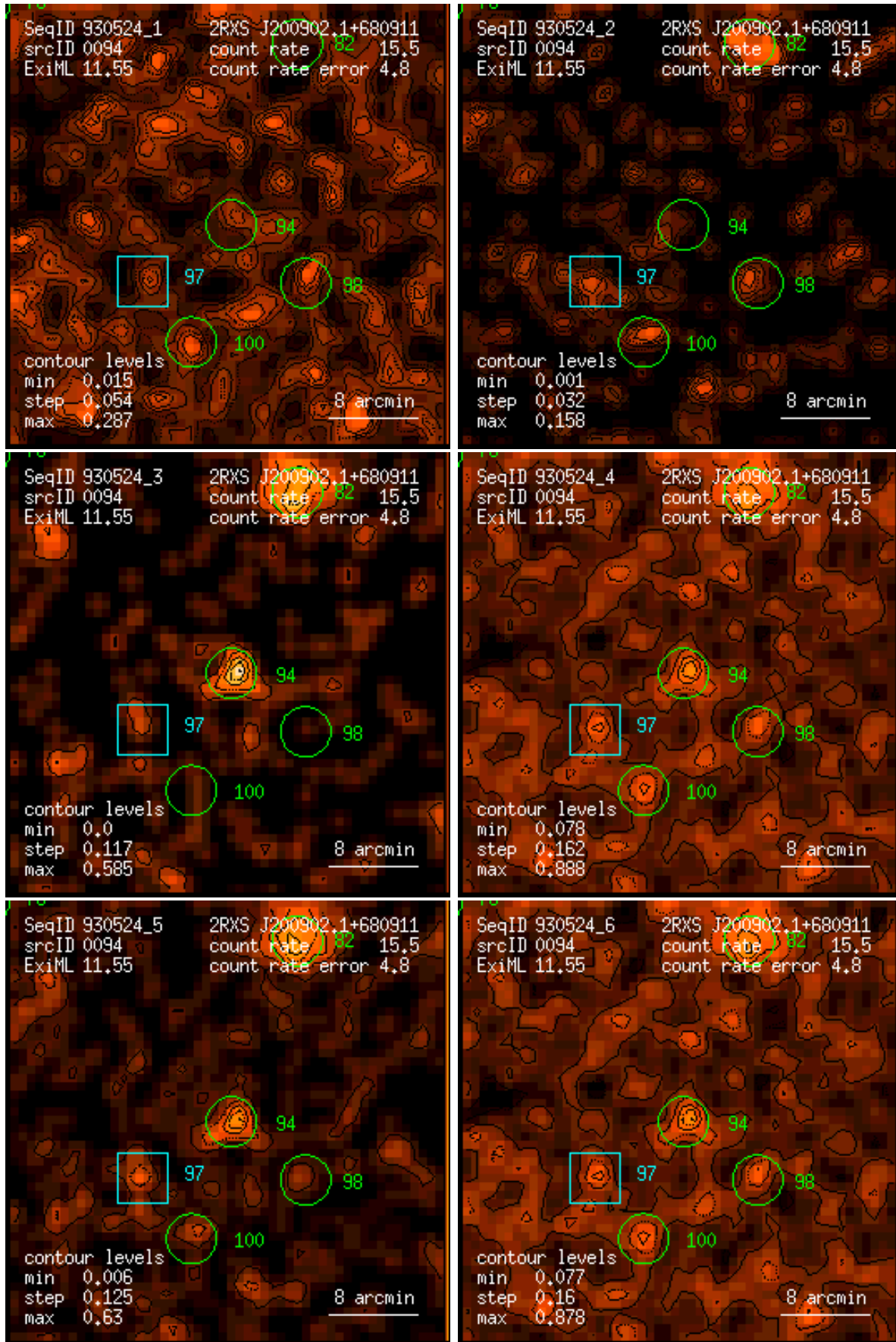
Figure 94: RASS 930524: detection 0094: band rate images, Gaussian filter: (1) PSPC channels 11 – 41, (2) 52 – 90, (3) 91 – 201, (4) 11 – 235, (5) 52 – 201, (6) 11 – 201. Broad band rates in counts/ks. Band rate contour levels in counts/ks/arcmin 2 .
