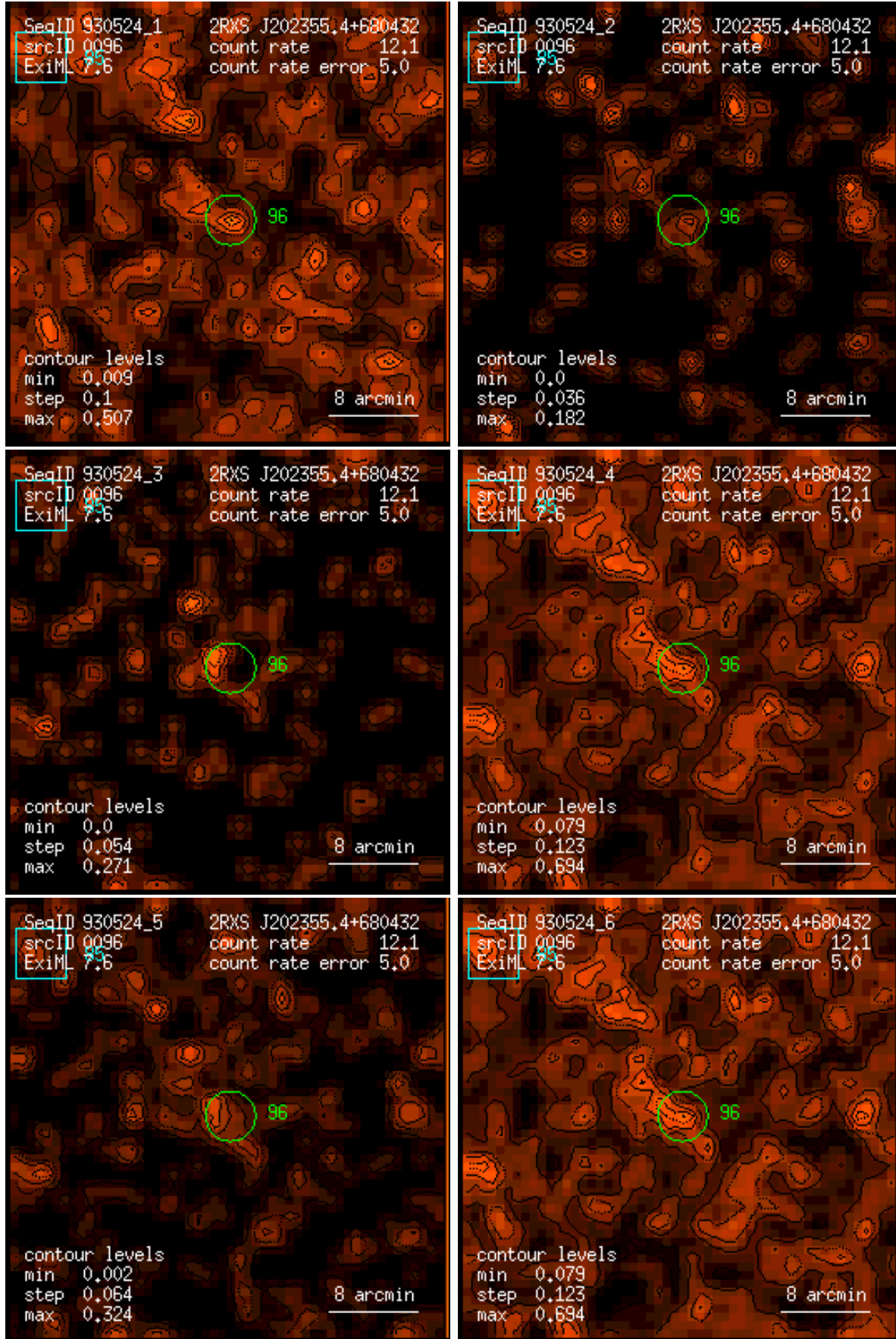
Figure 96: RASS 930524: detection 0096: band rate images, Gaussian filter: (1) PSPC channels 11 – 41, (2) 52 – 90, (3) 91 – 201, (4) 11 – 235, (5) 52 – 201, (6) 11 – 201. Broad band rates in counts/ks. Band rate contour levels in counts/ks/arcmin 2 .
