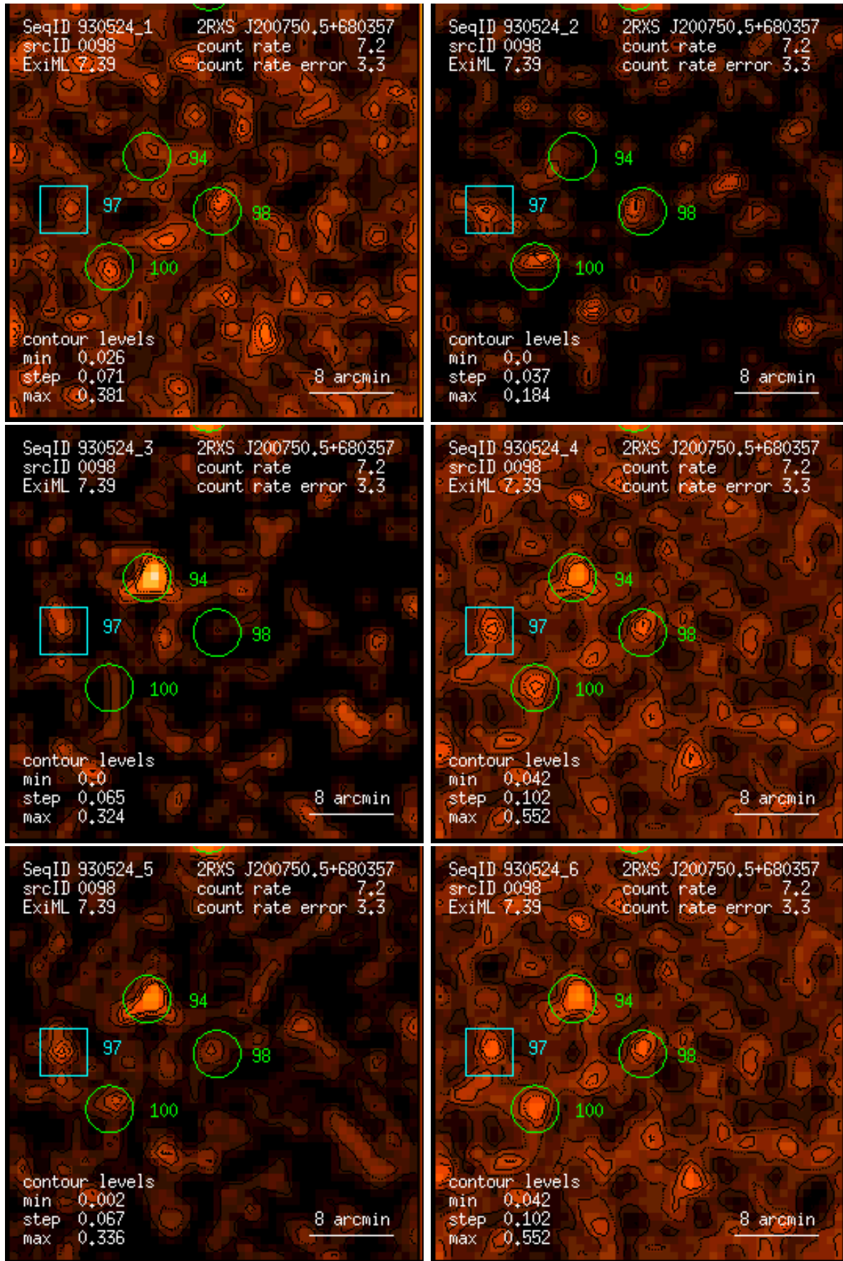
Figure 98: RASS 930524: detection 0098: band rate images, Gaussian filter: (1) PSPC channels 11 – 41, (2) 52 – 90, (3) 91 – 201, (4) 11 – 235, (5) 52 – 201, (6) 11 – 201. Broad band rates in counts/ks. Band rate contour levels in counts/ks/arcmin 2 .
