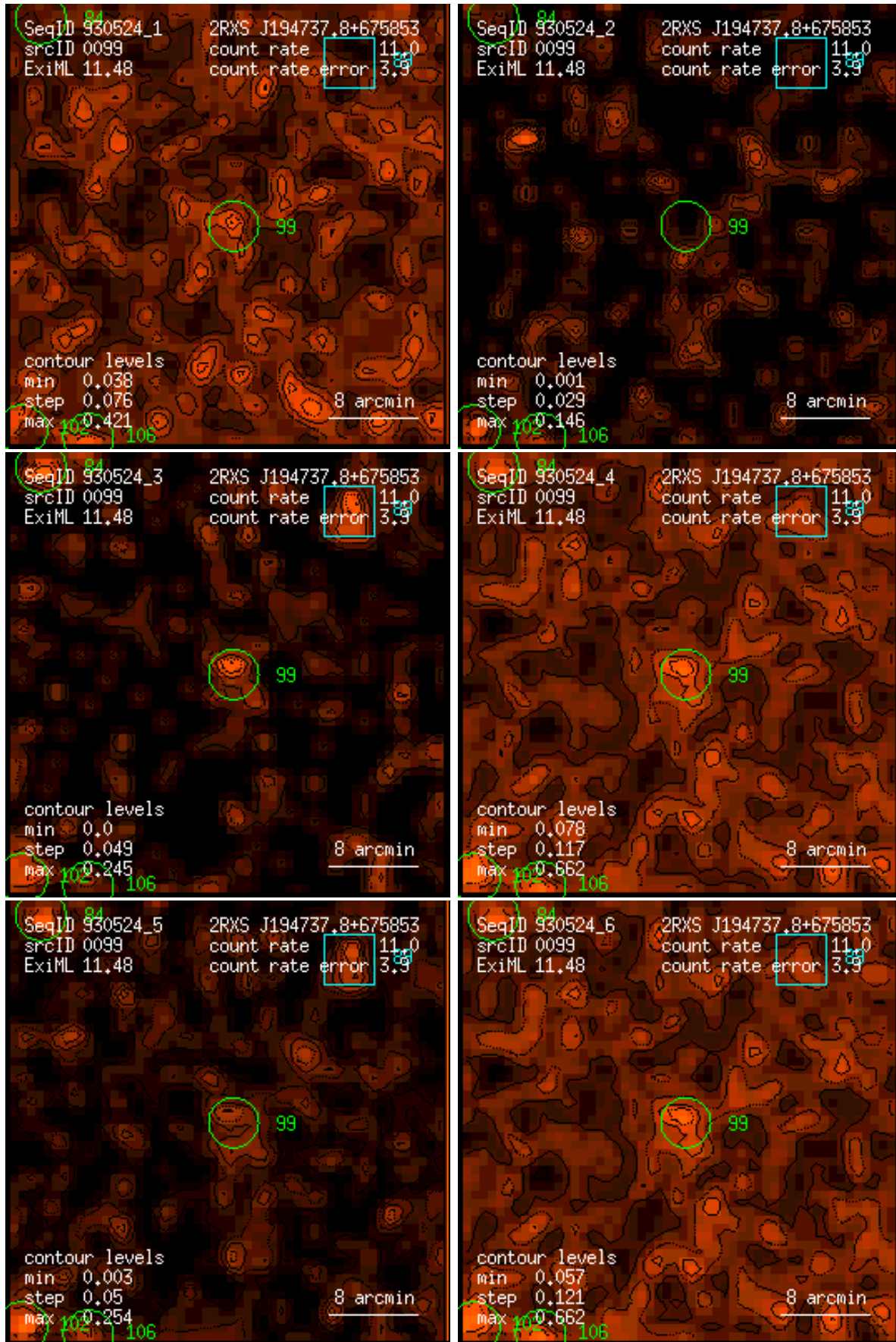
Figure 99: RASS 930524: detection 0099: band rate images, Gaussian filter: (1) PSPC channels 11 – 41, (2) 52 – 90, (3) 91 – 201, (4) 11 – 235, (5) 52 – 201, (6) 11 – 201. Broad band rates in counts/ks. Band rate contour levels in counts/ks/arcmin 2 .
