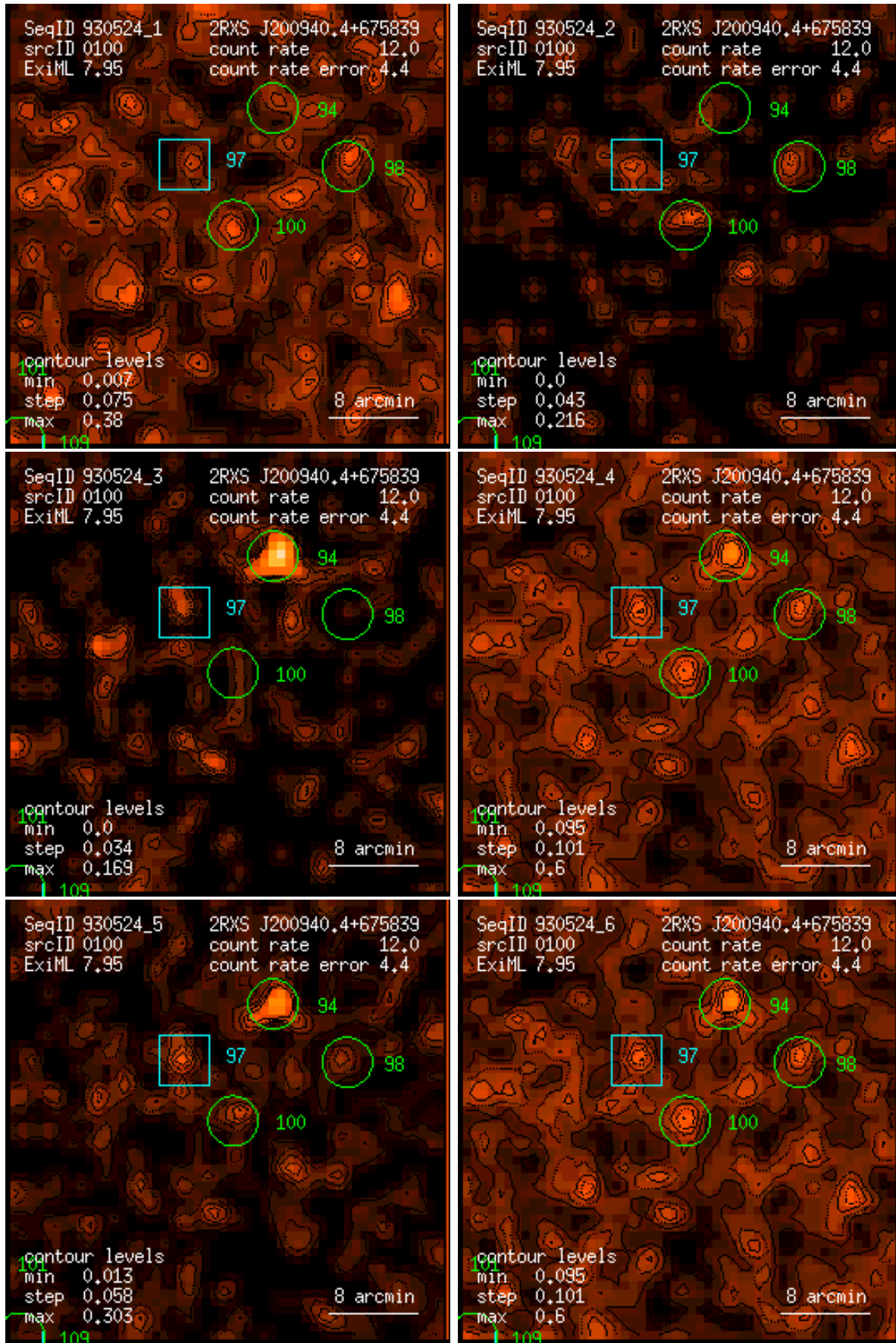
Figure 100: RASS 930524: detection 0100: band rate images, Gaussian filter: (1) PSPC channels 11 – 41, (2) 52 – 90, (3) 91 – 201, (4) 11 – 235, (5) 52 – 201, (6) 11 – 201. Broad band rates in counts/ks. Band rate contour levels in counts/ks/arcmin 2 .
