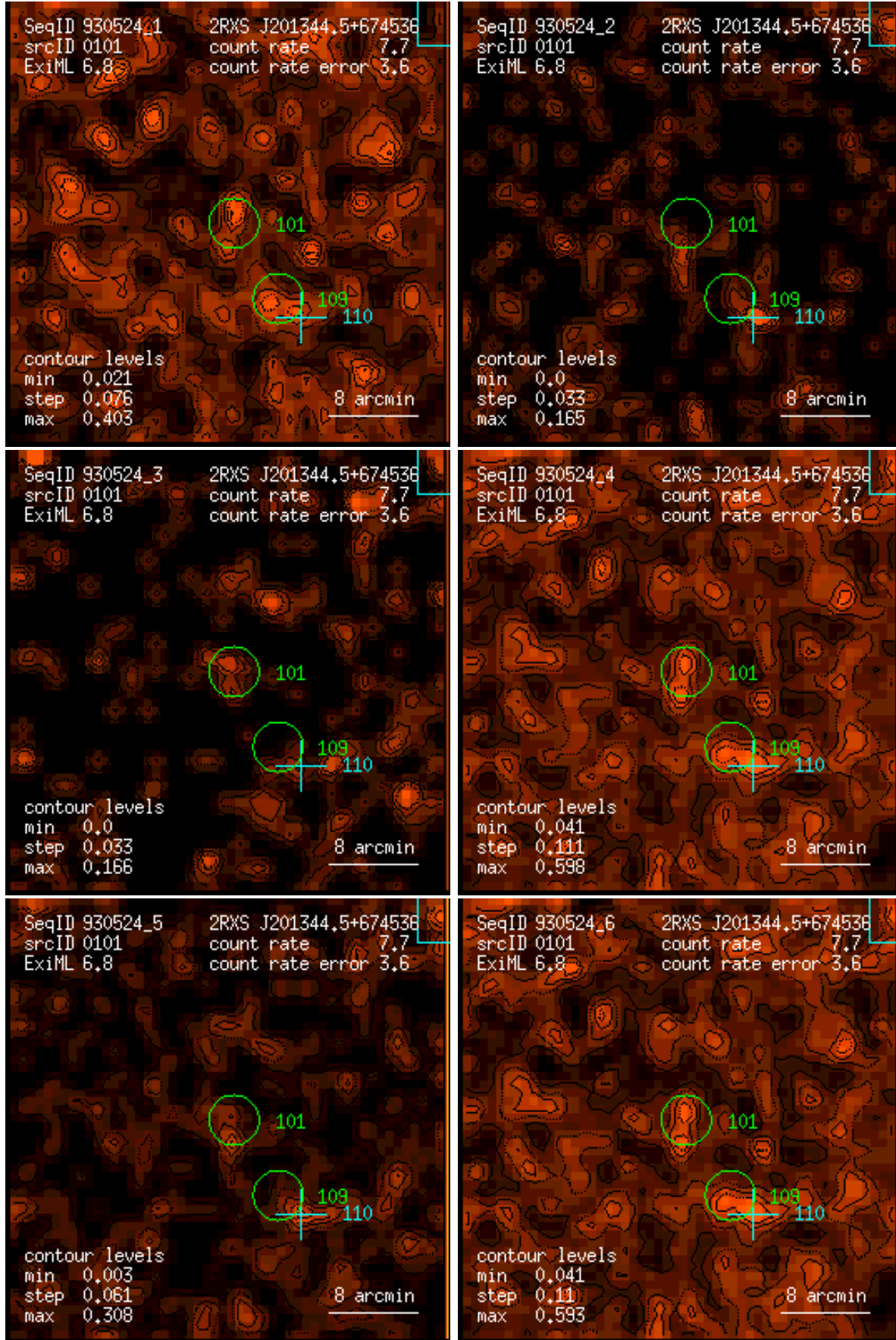
Figure 101: RASS 930524: detection 0101: band rate images, Gaussian filter: (1) PSPC channels 11 – 41, (2) 52 – 90, (3) 91 – 201, (4) 11 – 235, (5) 52 – 201, (6) 11 – 201. Broad band rates in counts/ks. Band rate contour levels in counts/ks/arcmin 2 .
