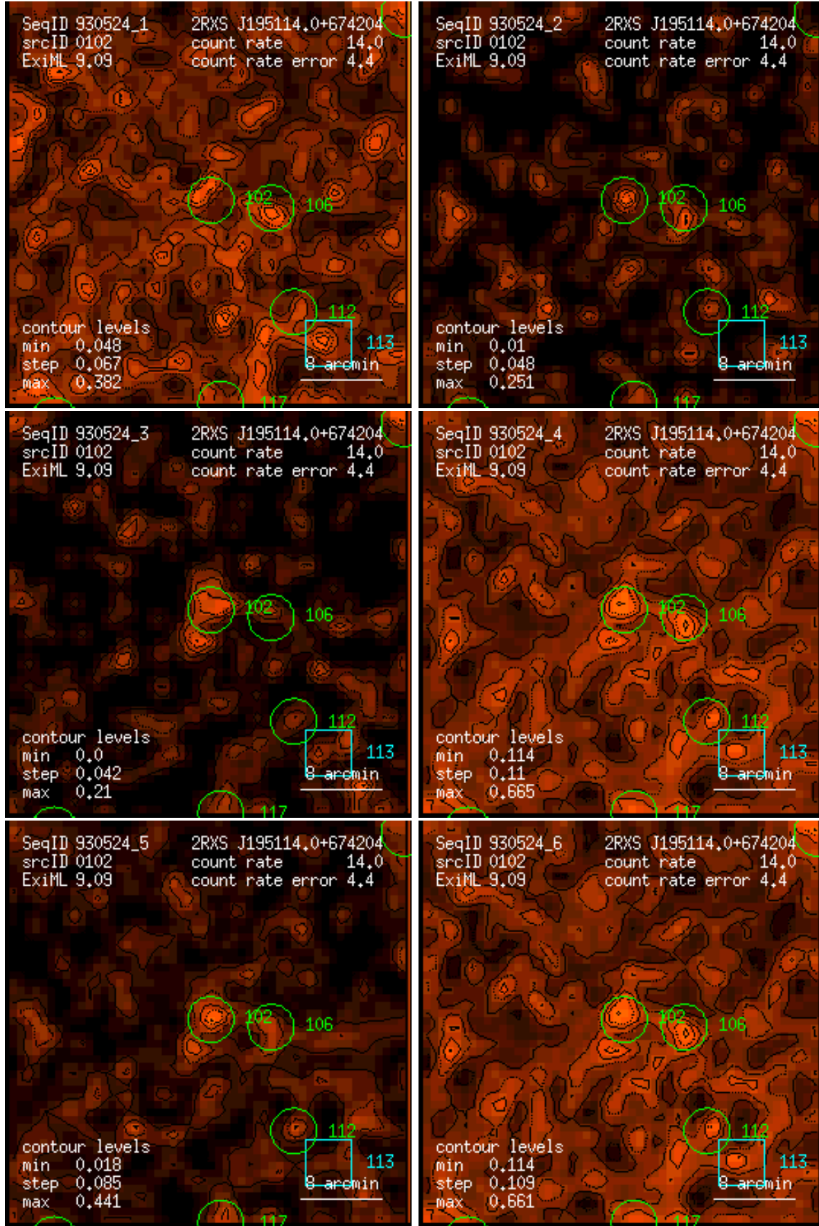
Figure 102: RASS 930524: detection 0102: band rate images, Gaussian filter: (1) PSPC channels 11 – 41, (2) 52 – 90, (3) 91 – 201, (4) 11 – 235, (5) 52 – 201, (6) 11 – 201. Broad band rates in counts/ks. Band rate contour levels in counts/ks/arcmin 2 .
