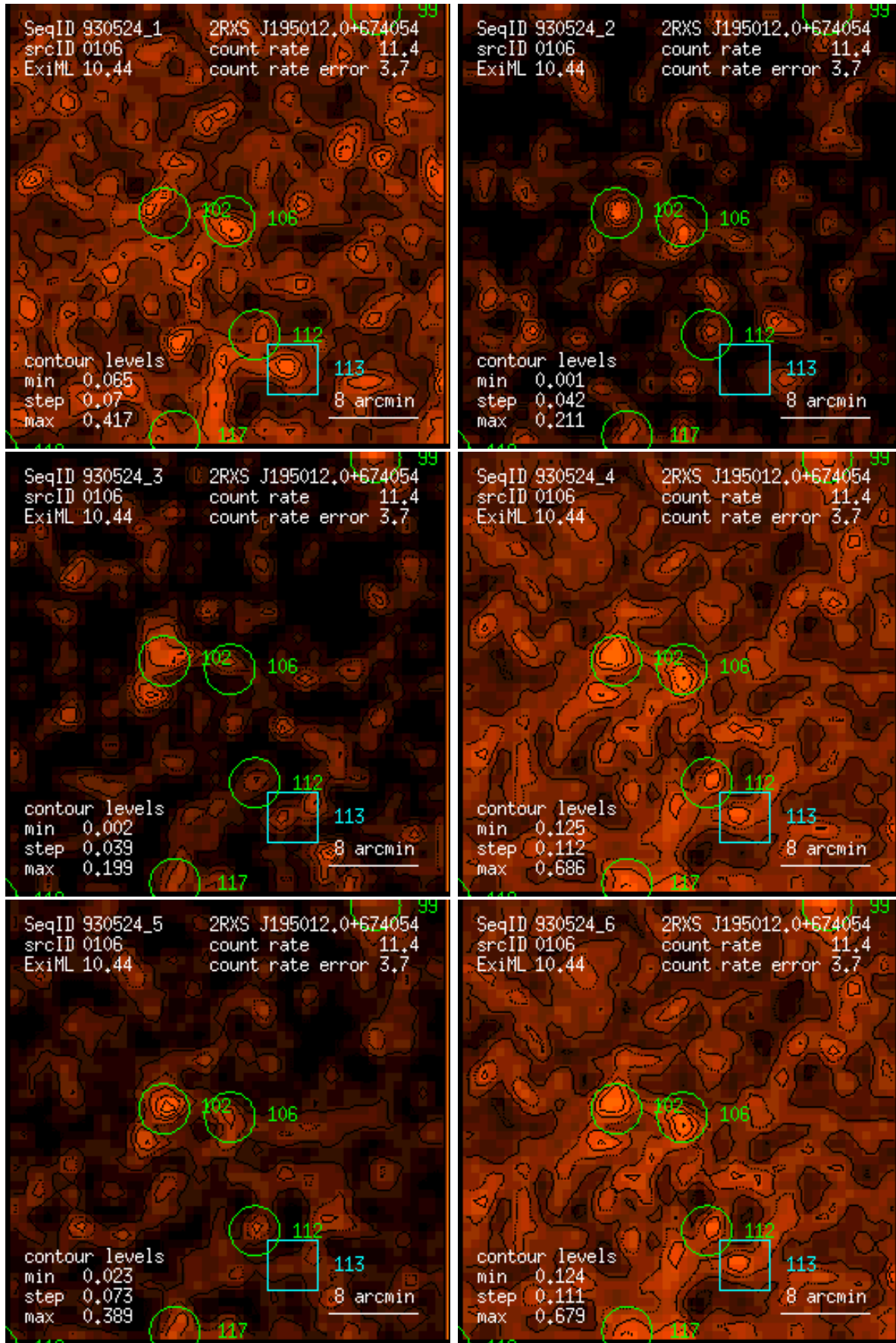
Figure 106: RASS 930524: detection 0106: band rate images, Gaussian filter: (1) PSPC channels 11 – 41, (2) 52 – 90, (3) 91 – 201, (4) 11 – 235, (5) 52 – 201, (6) 11 – 201. Broad band rates in counts/ks. Band rate contour levels in counts/ks/arcmin 2 .
