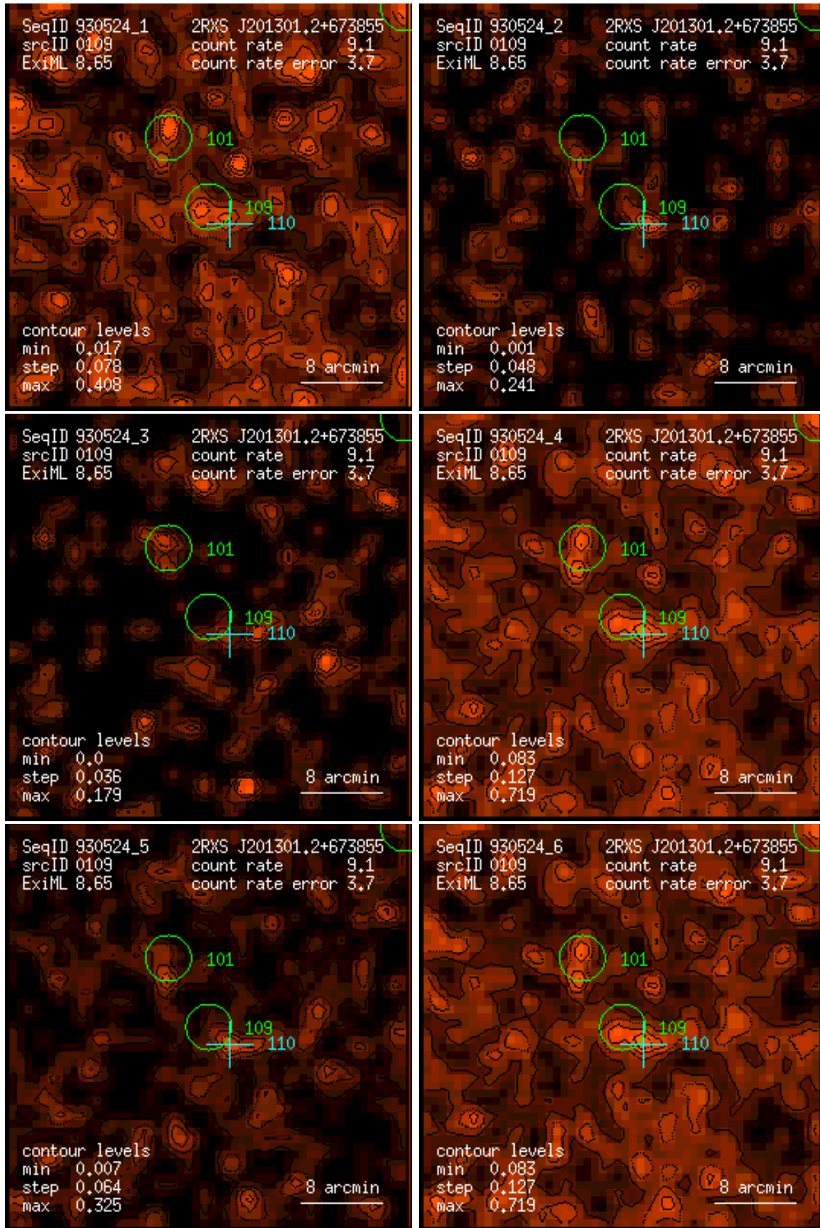
Figure 109: RASS 930524: detection 0109: band rate images, Gaussian filter: (1) PSPC channels 11 – 41, (2) 52 – 90, (3) 91 – 201, (4) 11 – 235, (5) 52 – 201, (6) 11 – 201. Broad band rates in counts/ks. Band rate contour levels in counts/ks/arcmin 2 .
