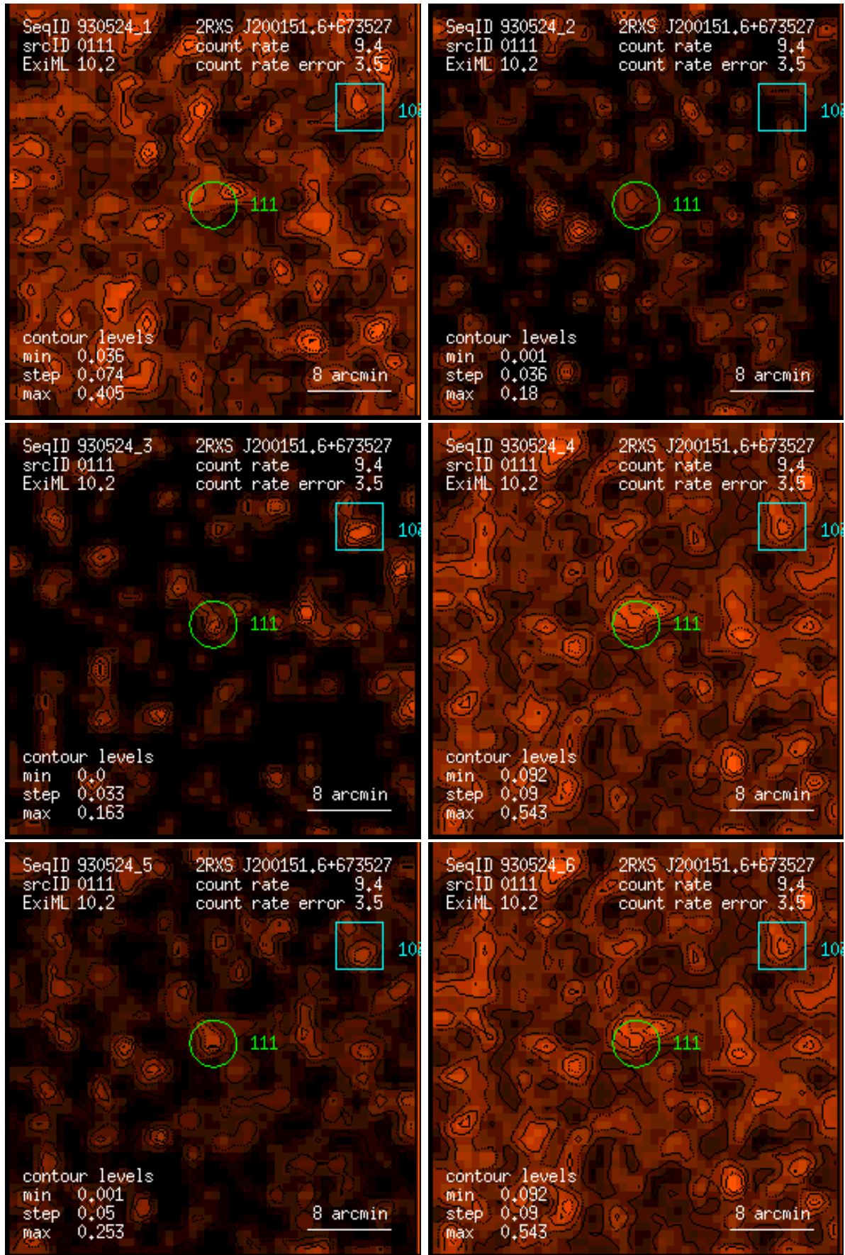
Figure 111: RASS 930524: detection 0111: band rate images, Gaussian filter: (1) PSPC channels 11 – 41, (2) 52 – 90, (3) 91 – 201, (4) 11 – 235, (5) 52 – 201, (6) 11 – 201. Broad band rates in counts/ks. Band rate contour levels in counts/ks/arcmin 2 .
