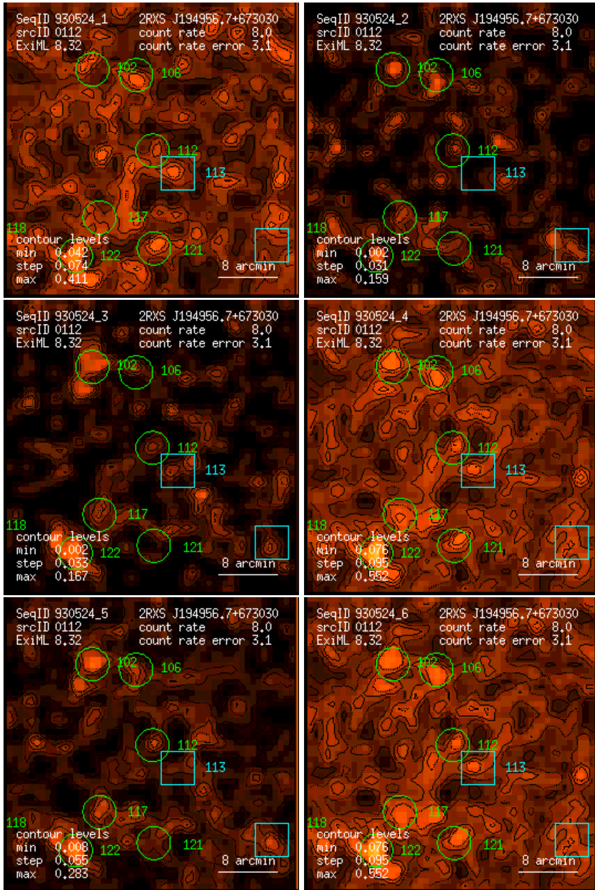
Figure 112: RASS 930524: detection 0112: band rate images, Gaussian filter: (1) PSPC channels 11 – 41, (2) 52 – 90, (3) 91 – 201, (4) 11 – 235, (5) 52 – 201, (6) 11 – 201. Broad band rates in counts/ks. Band rate contour levels in counts/ks/arcmin 2 .
