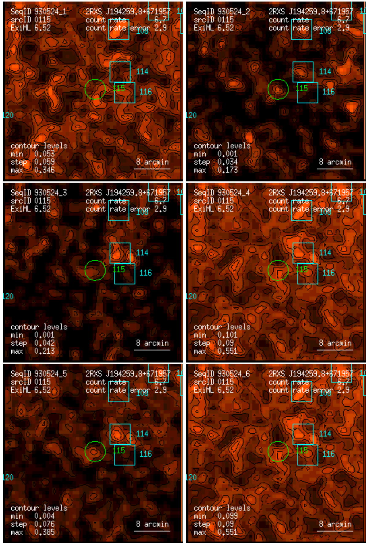
Figure 115: RASS 930524: detection 0115: band rate images, Gaussian filter: (1) PSPC channels 11 – 41, (2) 52 – 90, (3) 91 – 201, (4) 11 – 235, (5) 52 – 201, (6) 11 – 201. Broad band rates in counts/ks. Band rate contour levels in counts/ks/arcmin 2 .
