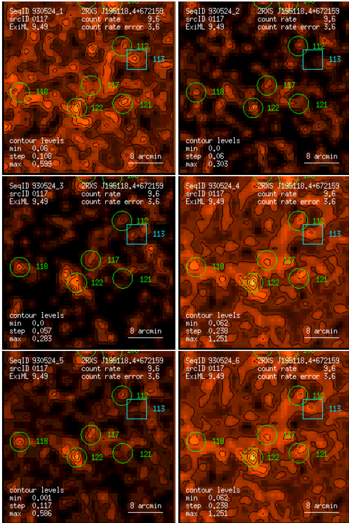
Figure 117: RASS 930524: detection 0117: band rate images, Gaussian filter: (1) PSPC channels 11 – 41, (2) 52 – 90, (3) 91 – 201, (4) 11 – 235, (5) 52 – 201, (6) 11 – 201. Broad band rates in counts/ks. Band rate contour levels in counts/ks/arcmin 2 .
