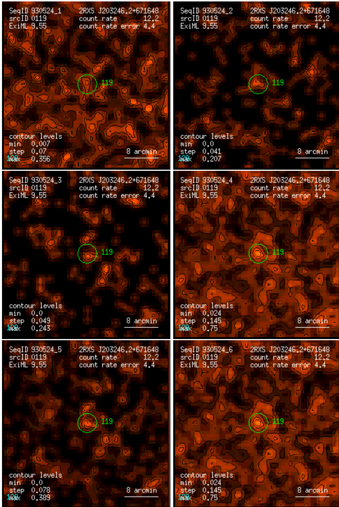
Figure 119: RASS 930524: detection 0119: band rate images, Gaussian filter: (1) PSPC channels 11 – 41, (2) 52 – 90, (3) 91 – 201, (4) 11 – 235, (5) 52 – 201, (6) 11 – 201. Broad band rates in counts/ks. Band rate contour levels in counts/ks/arcmin 2 .
