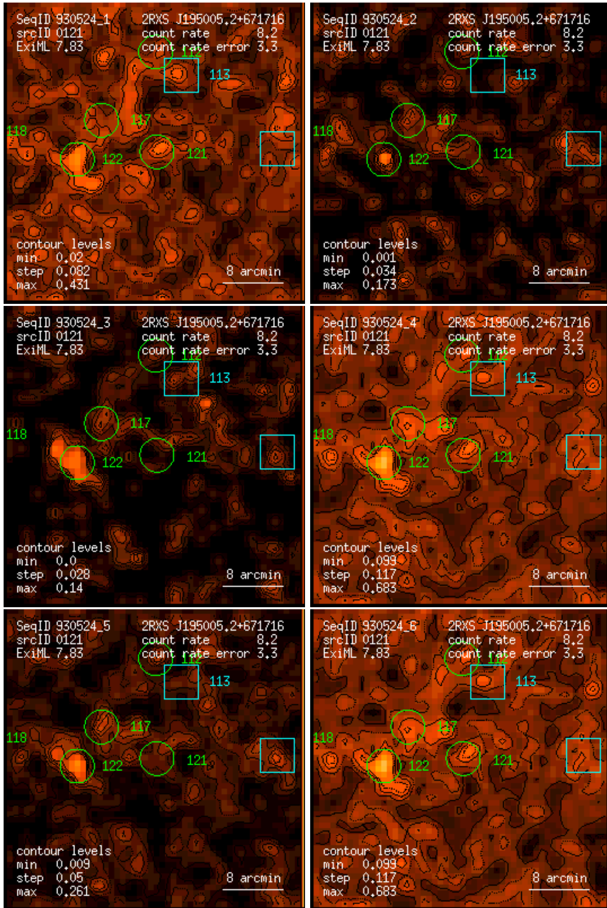
Figure 121: RASS 930524: detection 0121: band rate images, Gaussian filter: (1) PSPC channels 11 – 41, (2) 52 – 90, (3) 91 – 201, (4) 11 – 235, (5) 52 – 201, (6) 11 – 201. Broad band rates in counts/ks. Band rate contour levels in counts/ks/arcmin 2 .
