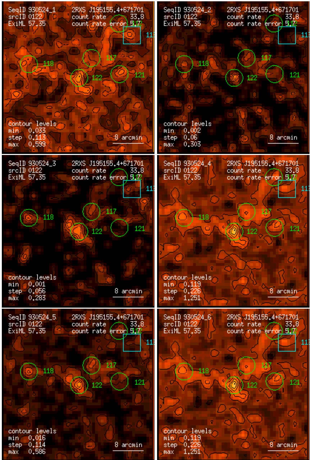
Figure 122: RASS 930524: detection 0122: band rate images, Gaussian filter: (1) PSPC channels 11 – 41, (2) 52 – 90, (3) 91 – 201, (4) 11 – 235, (5) 52 – 201, (6) 11 – 201. Broad band rates in counts/ks. Band rate contour levels in counts/ks/arcmin 2 .
