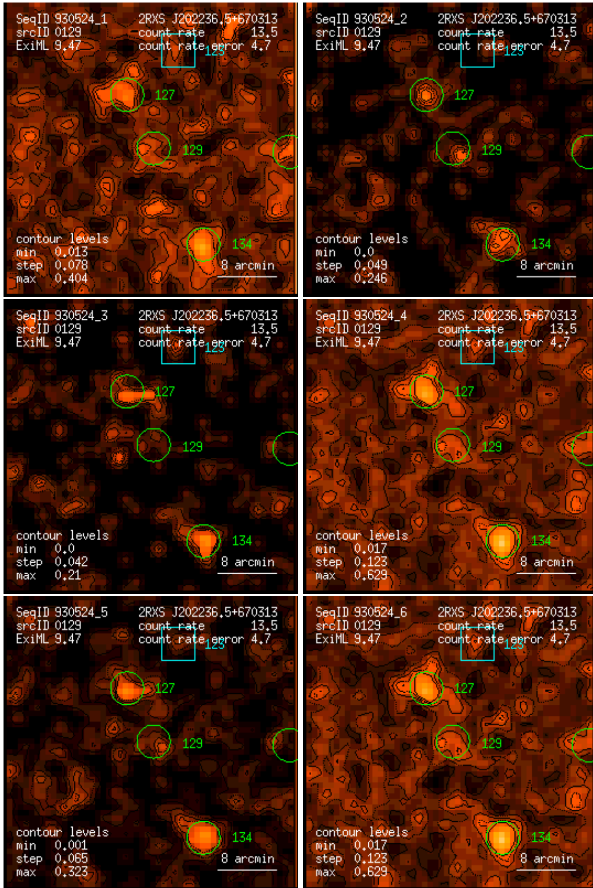
Figure 129: RASS 930524: detection 0129: band rate images, Gaussian filter: (1) PSPC channels 11 – 41, (2) 52 – 90, (3) 91 – 201, (4) 11 – 235, (5) 52 – 201, (6) 11 – 201. Broad band rates in counts/ks. Band rate contour levels in counts/ks/arcmin 2 .
