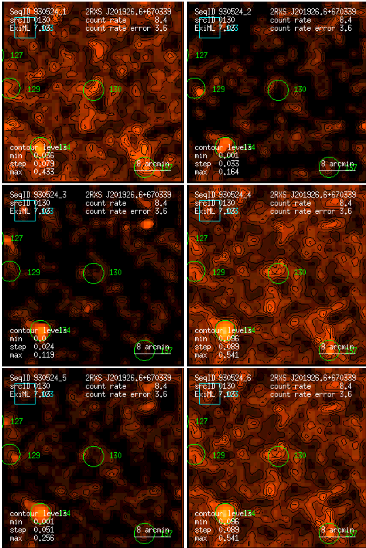
Figure 130: RASS 930524: detection 0130: band rate images, Gaussian filter: (1) PSPC channels 11 – 41, (2) 52 – 90, (3) 91 – 201, (4) 11 – 235, (5) 52 – 201, (6) 11 – 201. Broad band rates in counts/ks. Band rate contour levels in counts/ks/arcmin 2 .
