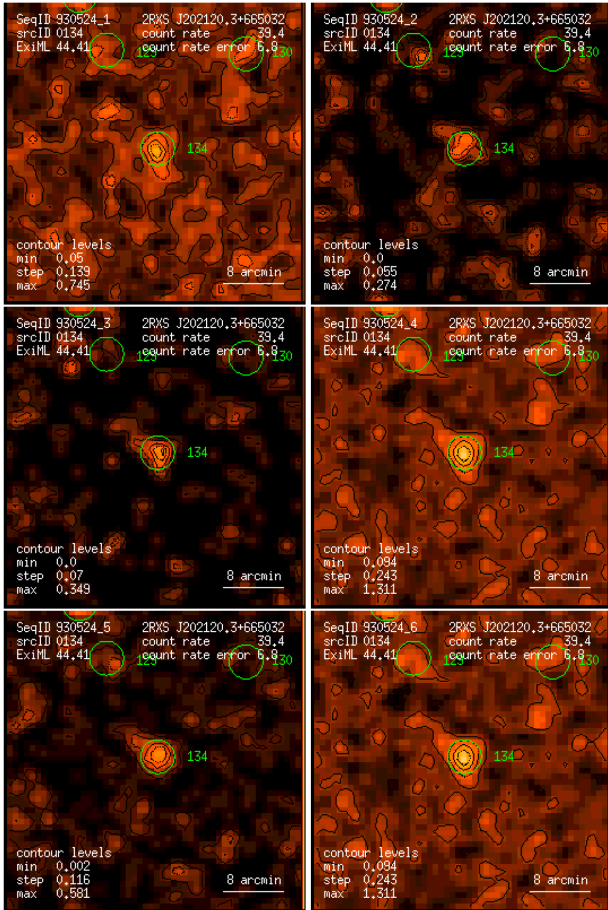
Figure 134: RASS 930524: detection 0134: band rate images, Gaussian filter: (1) PSPC channels 11 – 41, (2) 52 – 90, (3) 91 – 201, (4) 11 – 235, (5) 52 – 201, (6) 11 – 201. Broad band rates in counts/ks. Band rate contour levels in counts/ks/arcmin 2 .
