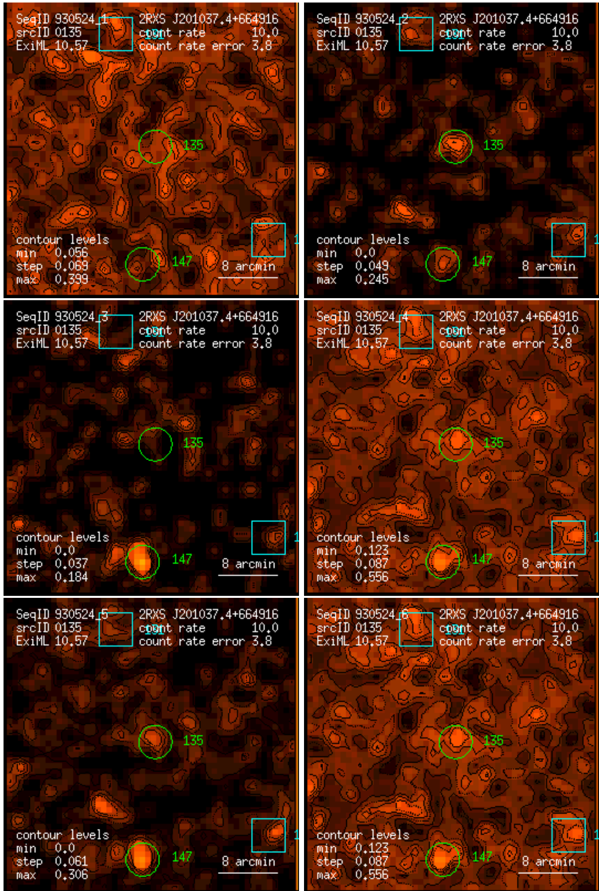
Figure 135: RASS 930524: detection 0135: band rate images, Gaussian filter: (1) PSPC channels 11 – 41, (2) 52 – 90, (3) 91 – 201, (4) 11 – 235, (5) 52 – 201, (6) 11 – 201. Broad band rates in counts/ks. Band rate contour levels in counts/ks/arcmin 2 .
