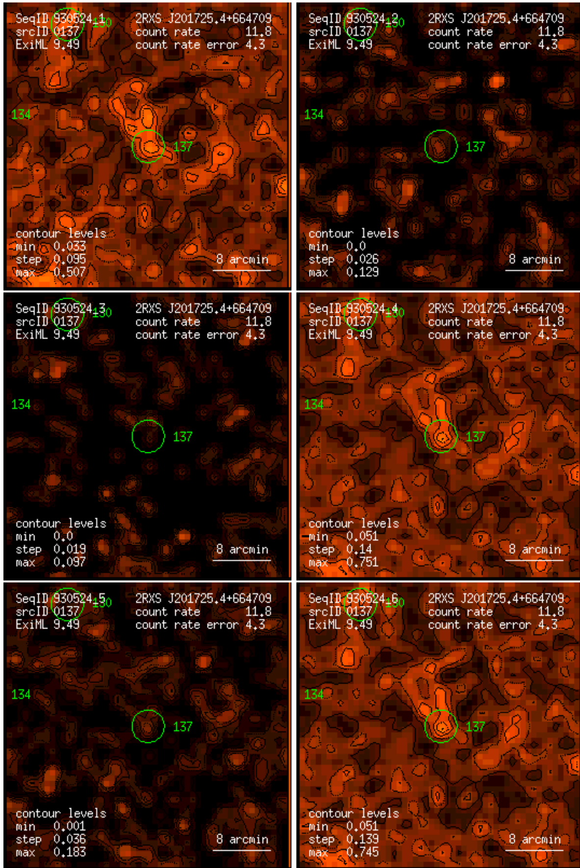
Figure 137: RASS 930524: detection 0137: band rate images, Gaussian filter: (1) PSPC channels 11 – 41, (2) 52 – 90, (3) 91 – 201, (4) 11 – 235, (5) 52 – 201, (6) 11 – 201. Broad band rates in counts/ks. Band rate contour levels in counts/ks/arcmin 2 .
