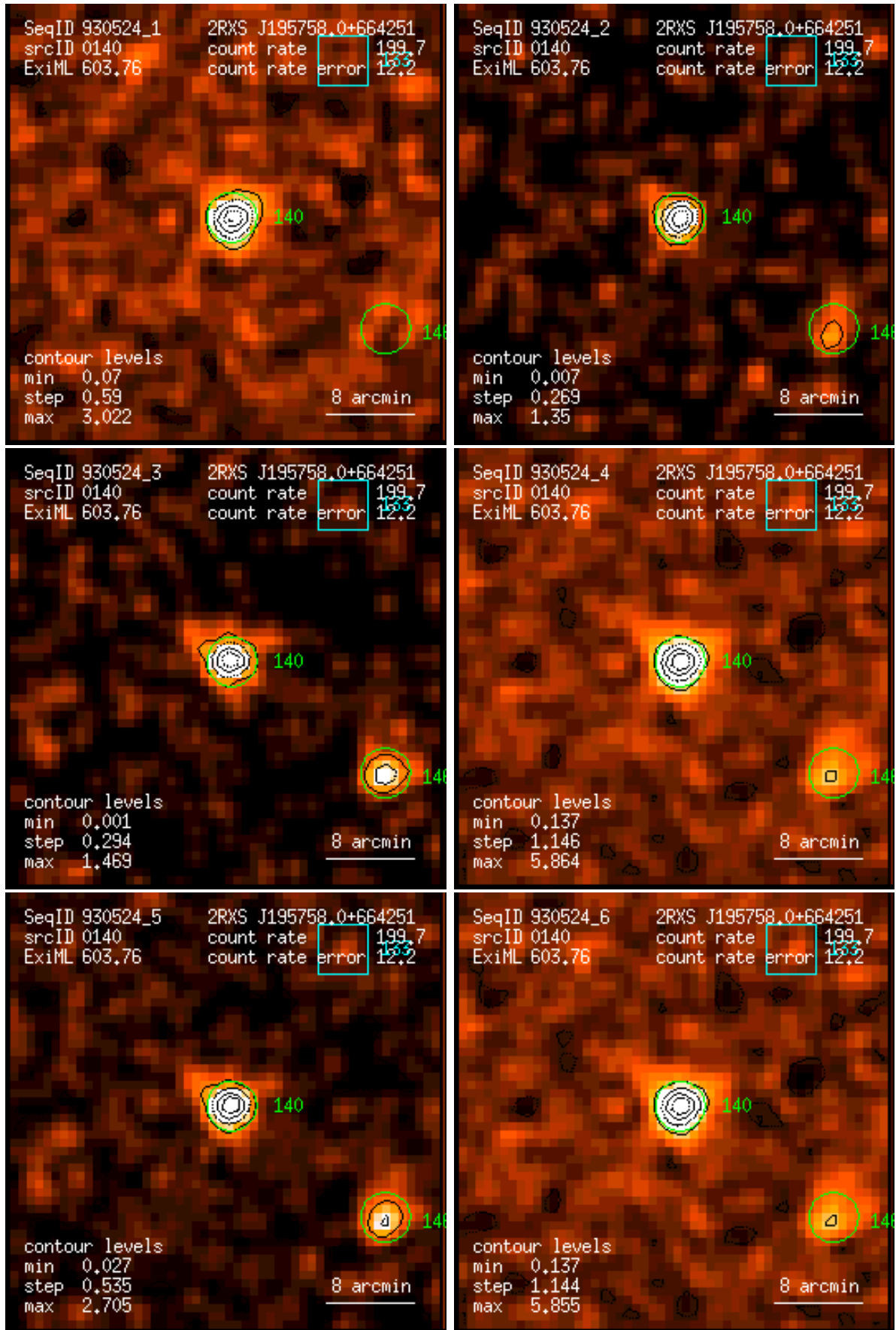
Figure 140: RASS 930524: detection 0140: band rate images, Gaussian filter: (1) PSPC channels 11 – 41, (2) 52 – 90, (3) 91 – 201, (4) 11 – 235, (5) 52 – 201, (6) 11 – 201. Broad band rates in counts/ks. Band rate contour levels in counts/ks/arcmin 2 .
