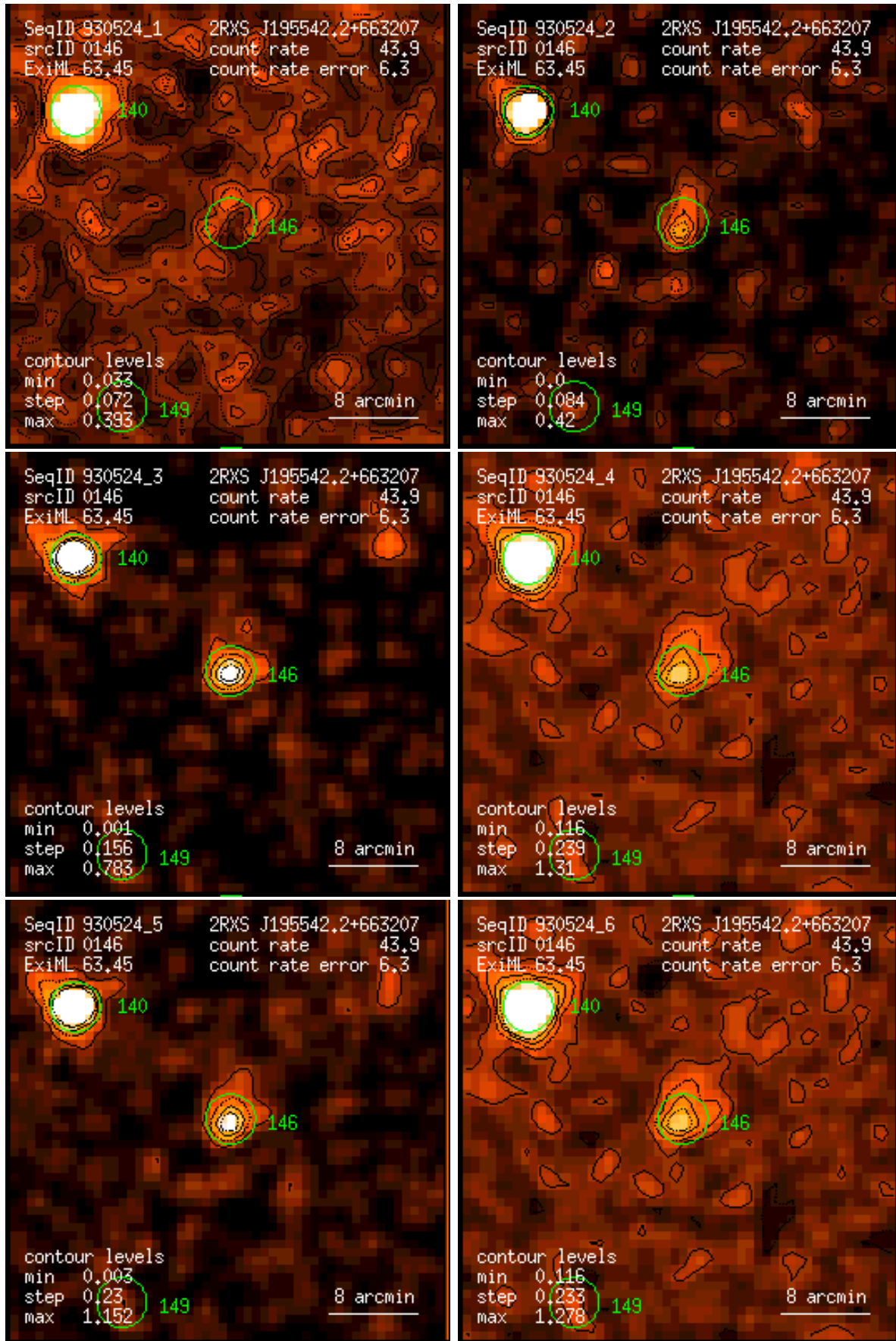
Figure 146: RASS 930524: detection 0146: band rate images, Gaussian filter: (1) PSPC channels 11 – 41, (2) 52 – 90, (3) 91 – 201, (4) 11 – 235, (5) 52 – 201, (6) 11 – 201. Broad band rates in counts/ks. Band rate contour levels in counts/ks/arcmin 2 .
