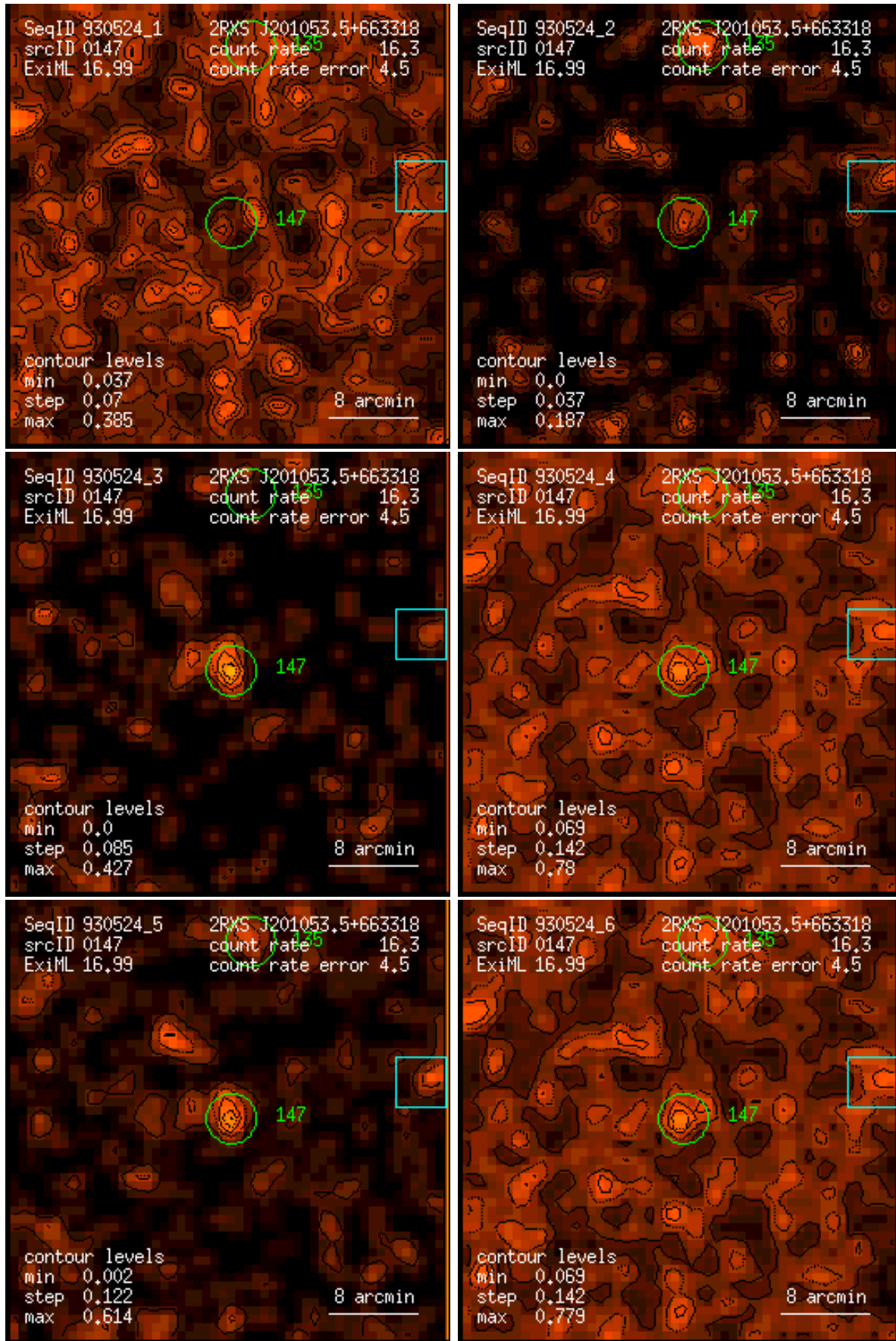
Figure 147: RASS 930524: detection 0147: band rate images, Gaussian filter: (1) PSPC channels 11 – 41, (2) 52 – 90, (3) 91 – 201, (4) 11 – 235, (5) 52 – 201, (6) 11 – 201. Broad band rates in counts/ks. Band rate contour levels in counts/ks/arcmin 2 .
