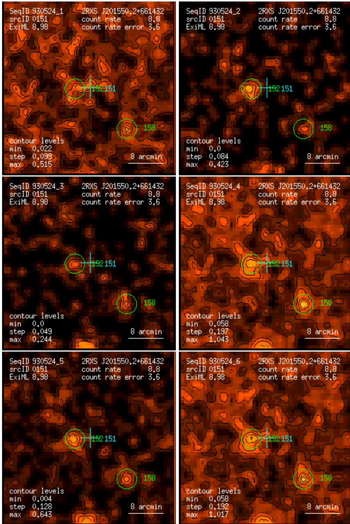
Figure 151: RASS 930524: detection 0151: band rate images, Gaussian filter: (1) PSPC channels 11 – 41, (2) 52 – 90, (3) 91 – 201, (4) 11 – 235, (5) 52 – 201, (6) 11 – 201. Broad band rates in counts/ks. Band rate contour levels in counts/ks/arcmin 2 .
