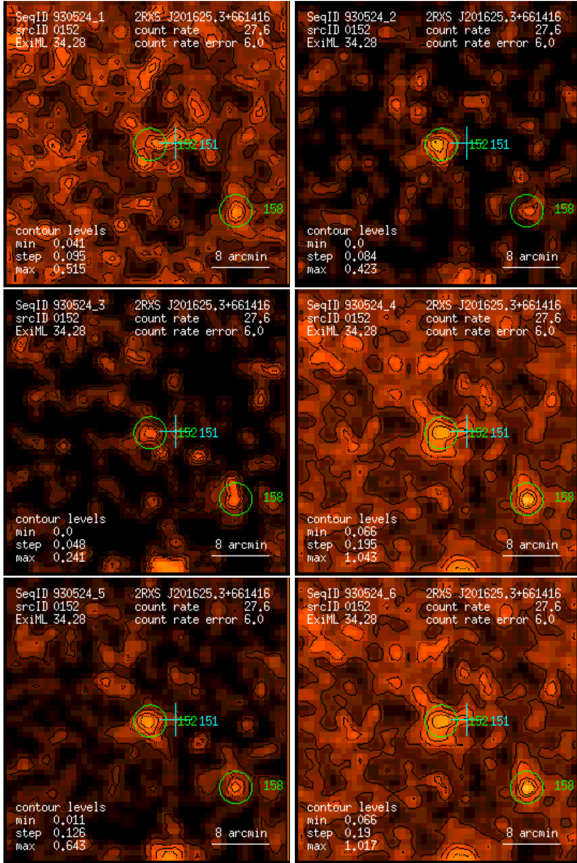
Figure 152: RASS 930524: detection 0152: band rate images, Gaussian filter: (1) PSPC channels 11 – 41, (2) 52 – 90, (3) 91 – 201, (4) 11 – 235, (5) 52 – 201, (6) 11 – 201. Broad band rates in counts/ks. Band rate contour levels in counts/ks/arcmin 2 .
