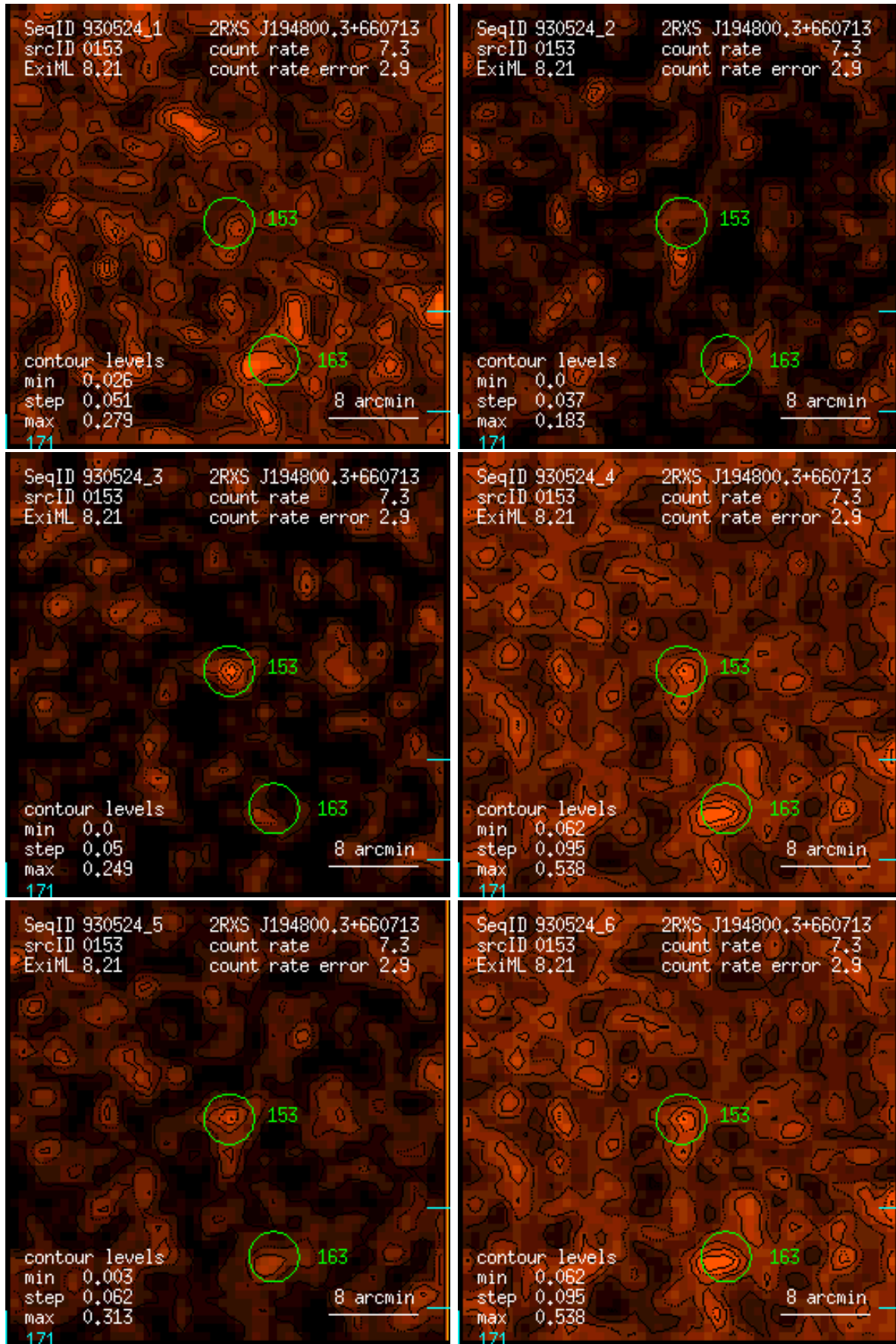
Figure 153: RASS 930524: detection 0153: band rate images, Gaussian filter: (1) PSPC channels 11 – 41, (2) 52 – 90, (3) 91 – 201, (4) 11 – 235, (5) 52 – 201, (6) 11 – 201. Broad band rates in counts/ks. Band rate contour levels in counts/ks/arcmin 2 .
