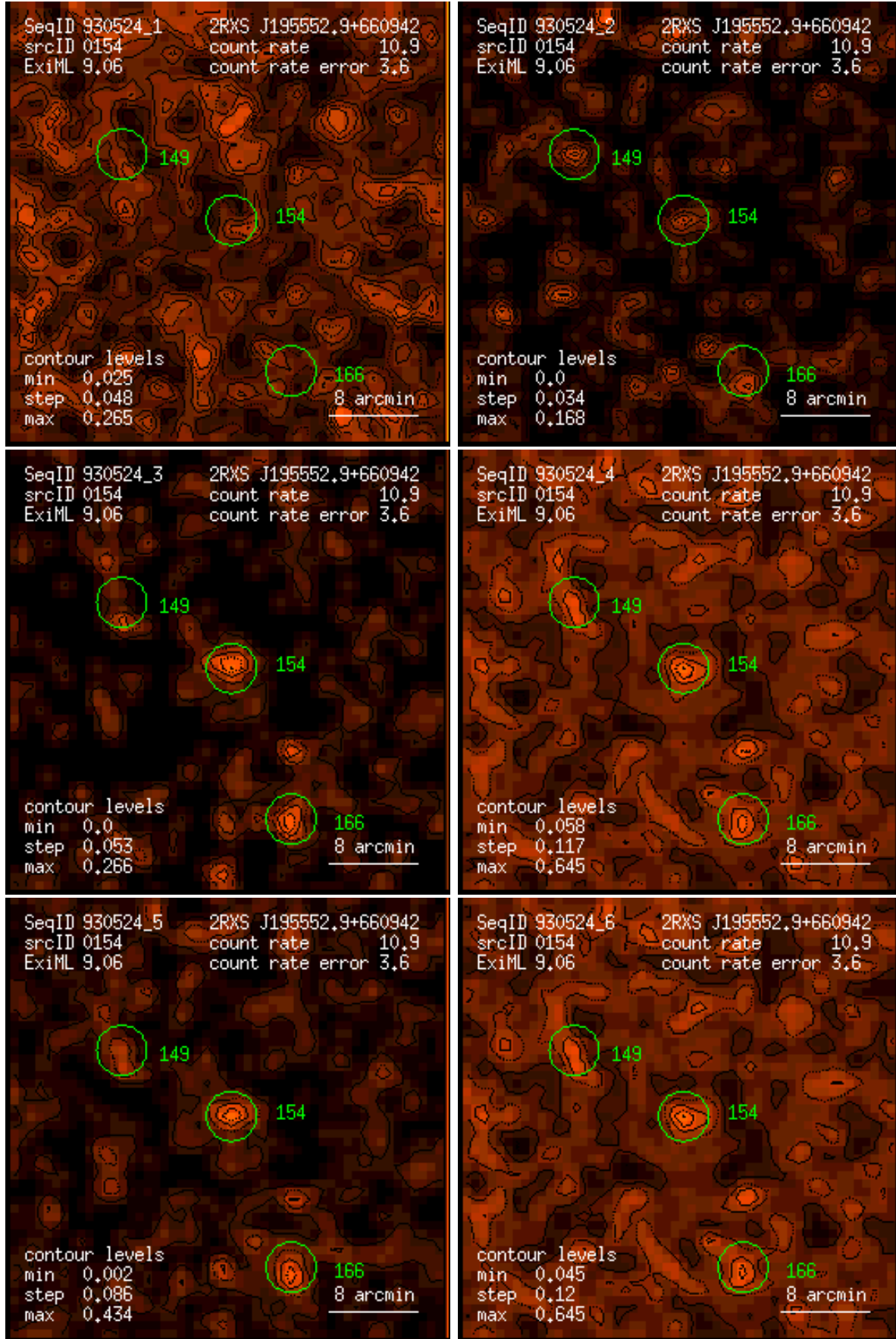
Figure 154: RASS 930524: detection 0154: band rate images, Gaussian filter: (1) PSPC channels 11 – 41, (2) 52 – 90, (3) 91 – 201, (4) 11 – 235, (5) 52 – 201, (6) 11 – 201. Broad band rates in counts/ks. Band rate contour levels in counts/ks/arcmin 2 .
