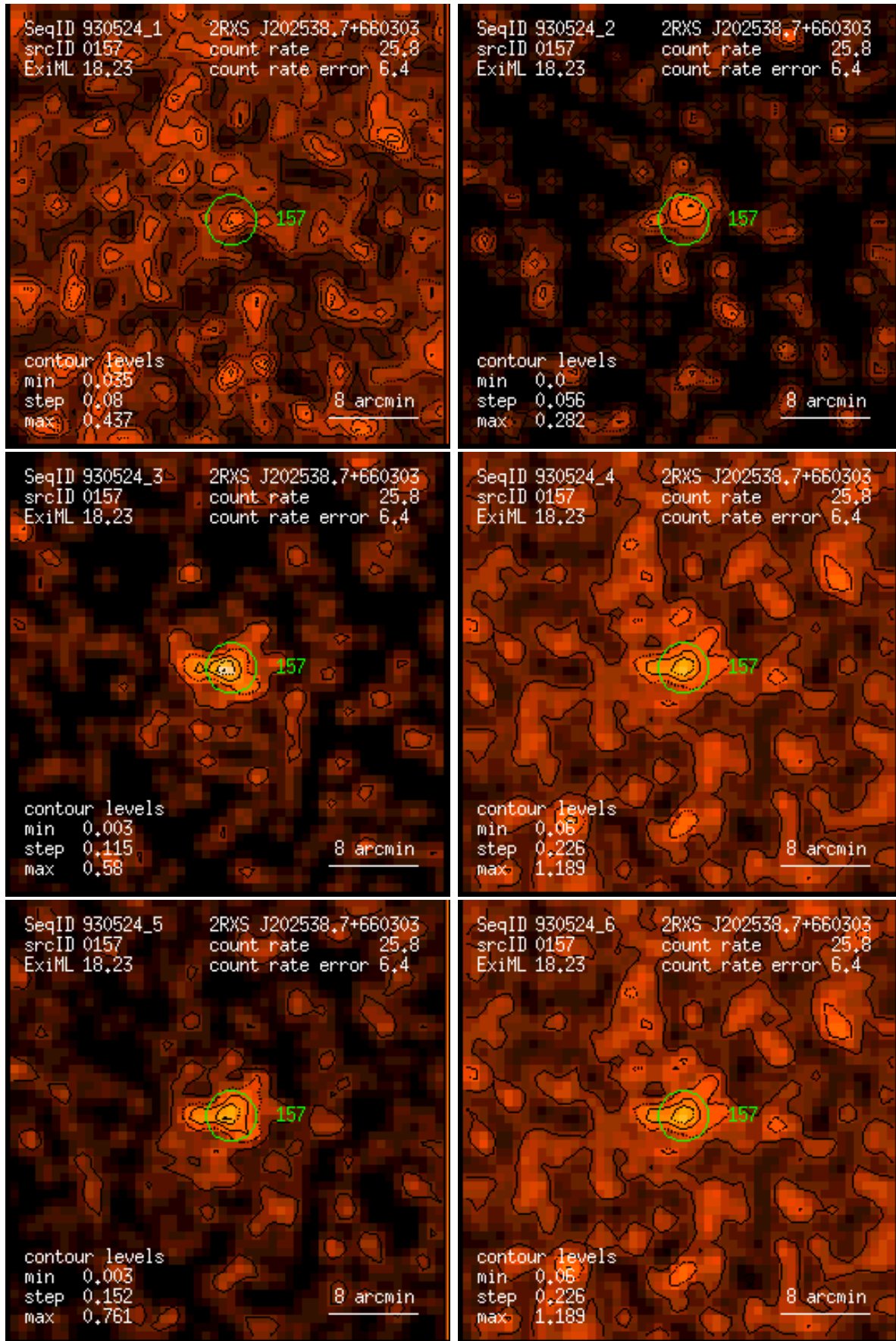
Figure 157: RASS 930524: detection 0157: band rate images, Gaussian filter: (1) PSPC channels 11 – 41, (2) 52 – 90, (3) 91 – 201, (4) 11 – 235, (5) 52 – 201, (6) 11 – 201. Broad band rates in counts/ks. Band rate contour levels in counts/ks/arcmin 2 .
