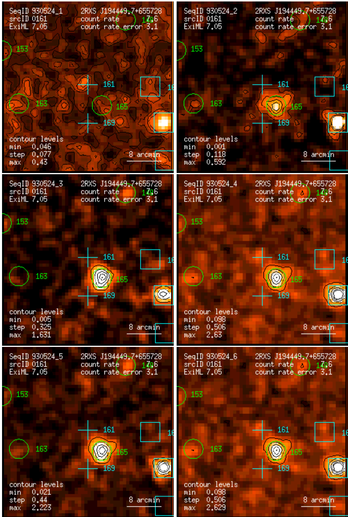
Figure 161: RASS 930524: detection 0161: band rate images, Gaussian filter: (1) PSPC channels 11 – 41, (2) 52 – 90, (3) 91 – 201, (4) 11 – 235, (5) 52 – 201, (6) 11 – 201. Broad band rates in counts/ks. Band rate contour levels in counts/ks/arcmin 2 .
