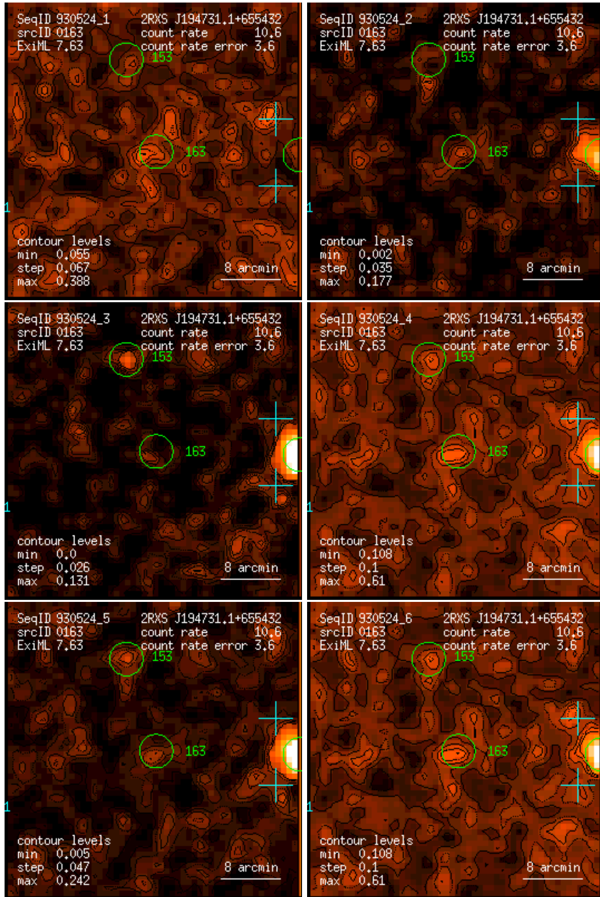
Figure 163: RASS 930524: detection 0163: band rate images, Gaussian filter: (1) PSPC channels 11 – 41, (2) 52 – 90, (3) 91 – 201, (4) 11 – 235, (5) 52 – 201, (6) 11 – 201. Broad band rates in counts/ks. Band rate contour levels in counts/ks/arcmin 2 .
