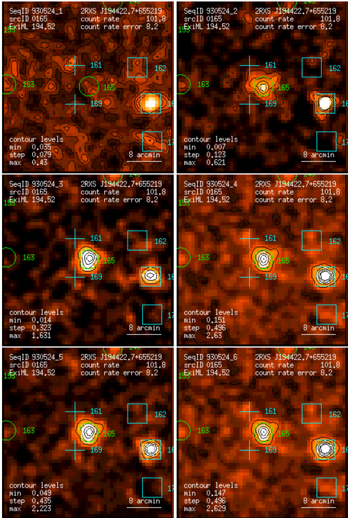
Figure 165: RASS 930524: detection 0165: band rate images, Gaussian filter: (1) PSPC channels 11 – 41, (2) 52 – 90, (3) 91 – 201, (4) 11 – 235, (5) 52 – 201, (6) 11 – 201. Broad band rates in counts/ks. Band rate contour levels in counts/ks/arcmin 2 .
